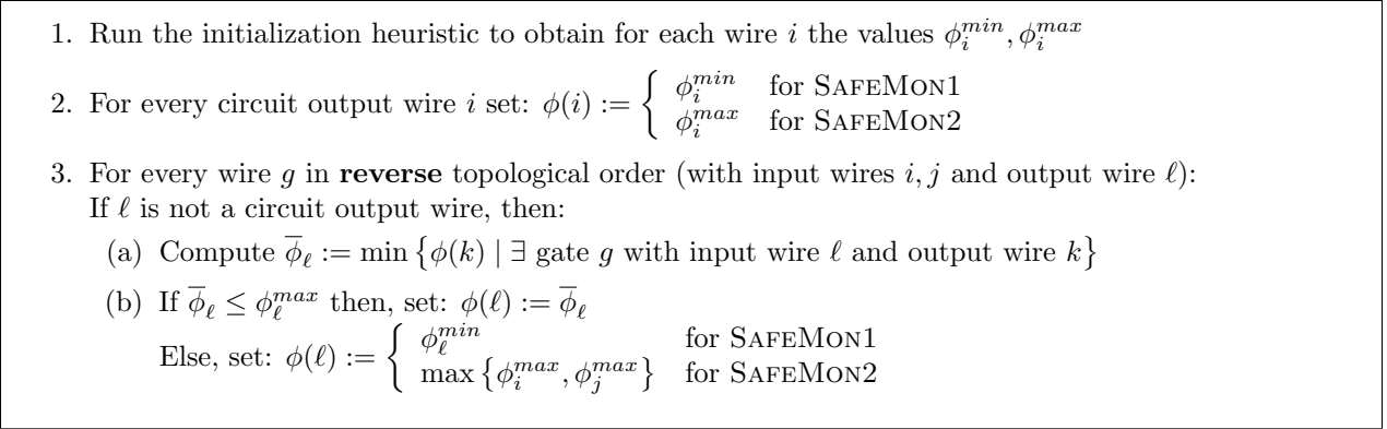
Figure 11: Heuristics for finding safe and monotone wire orderings
