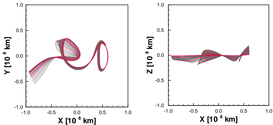
Figure 3.15. Evolution of Stable Manifold Along \alpha_d = 43^\circ
