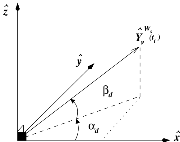
Figure 3.8. Characterization of Stable/Unstable Eigenvector Directions
