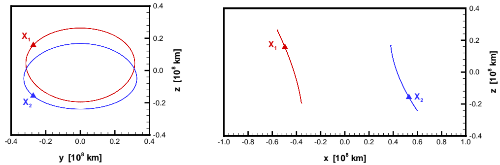
Figure 3.17. Similar L_1 and L_2 Orbits
