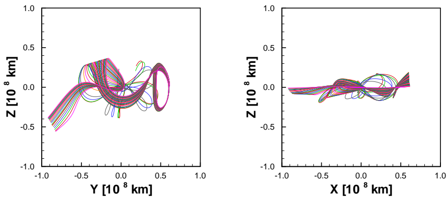
Figure 3.16. Evolution of Stable Manifold Along \alpha = 305^\circ
