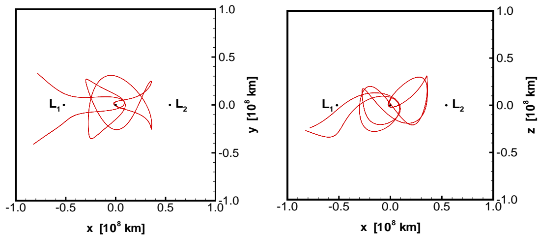
Figure 3.2. TSC of Helin-Roman-Crockett – Synodic Rotating Frame
