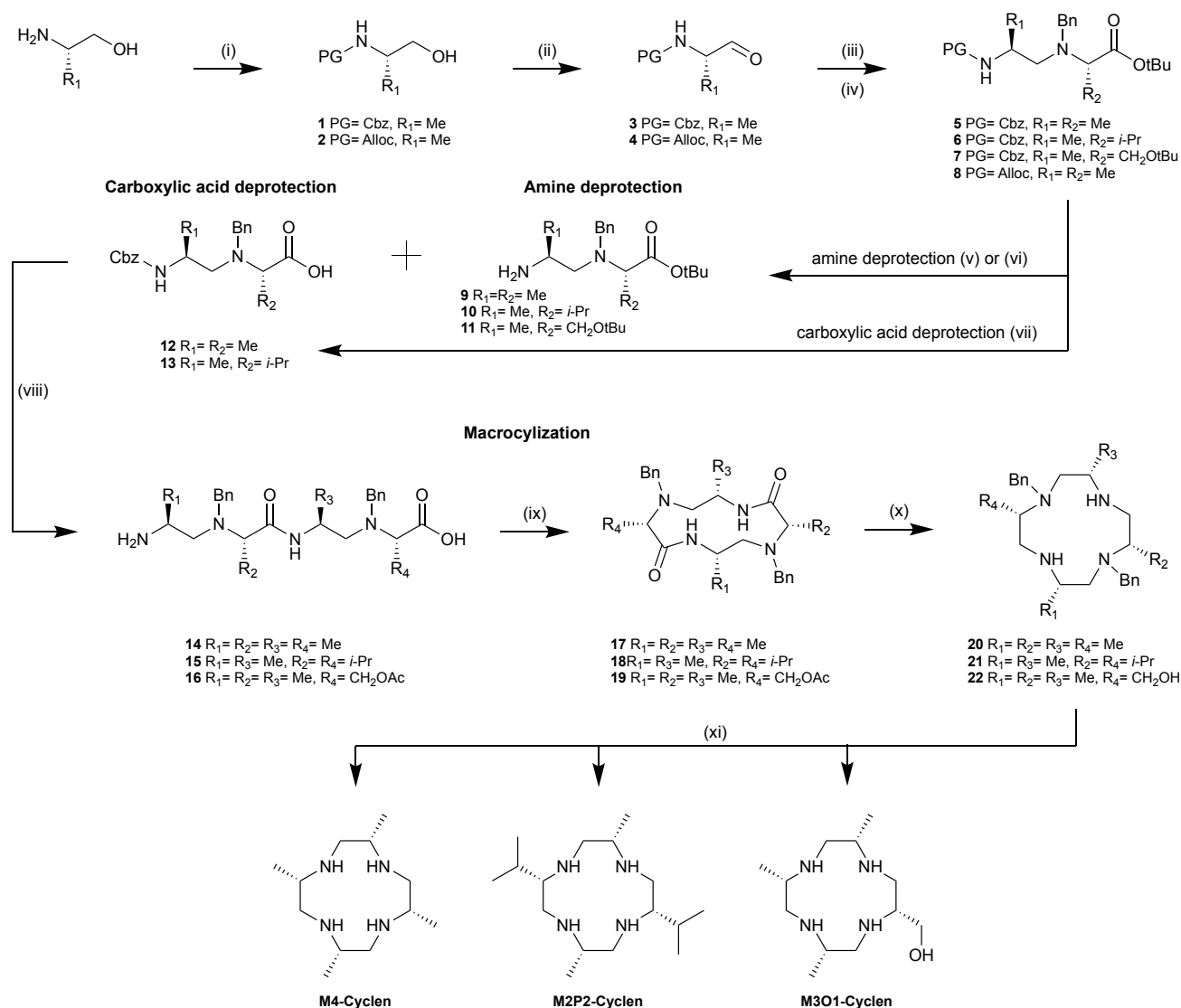
Scheme 1 Syntheses of 2 S ,5 S ,8 S ,11 S -2,5,8,11-Tetra-methyl-cyclen (M4-cyclen), 2 S ,5 S ,8 S ,11 S -2,8-Diisopropyl-5,11-di-methyl-cyclen (M2P2-cyclen) and 2 S ,5 S ,8 S ,11 S -2-hydroxymethyl-5,8,11-tri-methyl-cyclen (M3O1-cyclen). Reagents and conditions: (i) Cbz-Cl or Alloc-Cl, Na 2 CO 3 , EtOAc/H 2 O, RT, 1h; (ii) IBX, DMSO, EtOAc, reflux, 2-5h (iii) amine, NaBH(OAc) 3 , CH 2 Cl 2 , 20-25°C, 2-16h; (iv) BnBr, K 2 CO 3 , MeCN, 40-50°C, 8-16h; (v) PhSiH 3 , Pd(PPh 3 ) 4 , CH 2 Cl 2 , 20-25°C, 4h; (vi) Pd/BaSO 4 , H 2 , MeOH, 20-25°C, 4-16h; (vii) HCl in dioxane, 40°C, 16h; (viii) HATU, DIPEA, MeCN, 20-25°C, 2-4h; (ix) HBr in acetic acid 16 wt. %, 40°C, 30 min; (x) HATU, DIPEA, MeCN, 20-25°C, 20 min.; (xi) TMS-Cl, LiAlH 4 , THF/CH 2 Cl 2 , 0-5 °C → 20-25 °C, 3h; (xii) Pd/C, ammonium formate, EtOH, reflux, 16h or Pd/C, H 2 , MeOH, RT, 16h.
