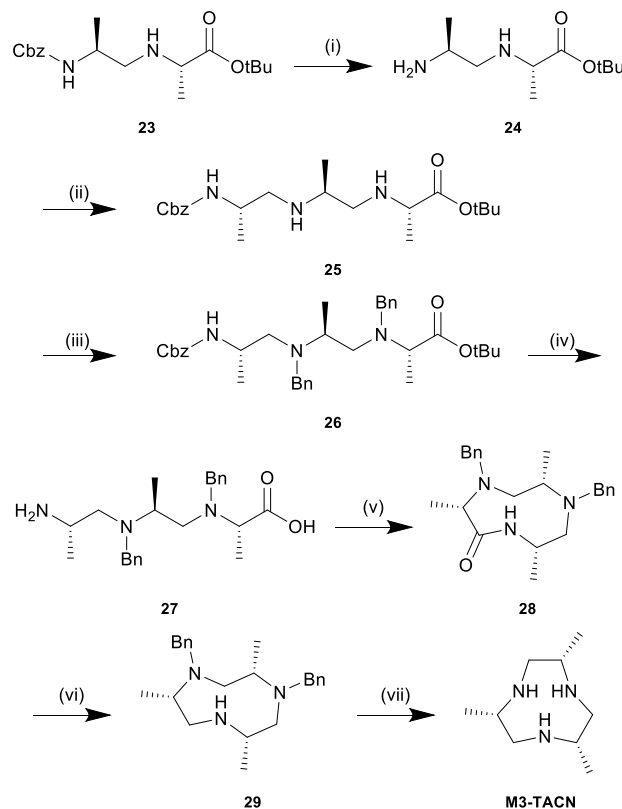
Scheme 2 Synthesis of M3TACN. Reagents and conditions: (i) Pd/C, H 2 , MeOH, 20-25°C, 4h; (ii) NaBH(OAc) 3 , CH 2 Cl 2 , 20-25°C, 16h; (iii) BnBr, K 2 CO 3 , MeCN, 20-25°C, 16h; (iv) HBr in acetic acid 16 wt. %, 40°C, 30 min; (v) HATU, DIPEA, MeCN, 20-25°C, 30 min.; (vi) TMS-Cl, LiAlH 4 , THF/CH 2 Cl 2 , 0-5 °C → 20-25 °C, 5h; (vii) Pd/C, ammonium formate, EtOH, reflux, 16h.
