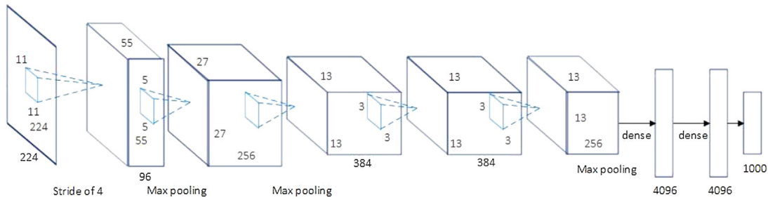
Fig. 2. AlexNet Convolutional Neural Network architecture.
