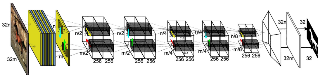
Fig. 18. Representation of ReSeg network. VGG-16 convolutional layers are represented by the blue and yellow first layers. The rest of the architecture is based on the ReNet approach with fine-tuning purposes. (For interpretation of the references to color in this figure legend, the reader is referred to the web version of the article.) Figure extracted from [83].
