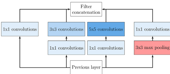
Fig. 4. Inception module with dimensionality reduction from the GoogLeNet architecture.
