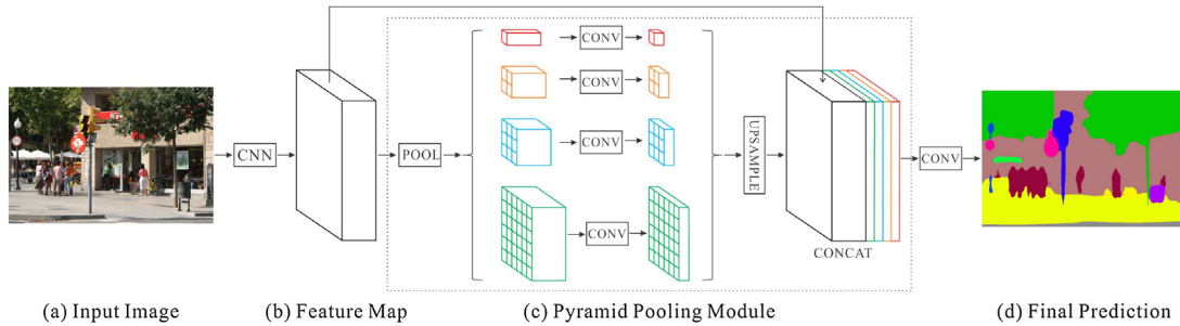
Fig. 17. PSPNet architecture. Initial feature maps (b) are extracted from input images (a) by using a pretrained ResNet [18] alongside dilated network strategy. Pyramid pooling module (c) covers from the whole, half to small regions of the image. Finally, initial feature map is concatenated with pooling module output and applying a convolution layer final predicted maps (d) are generated. Figure extracted from [82].
