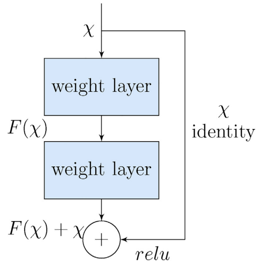
Fig. 5. Residual block from the ResNet architecture.
