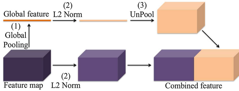
Fig. 16. ParseNet context module overview in which a global feature (from a previous layer) is combined with the feature of the next layer to add context information. Figure extracted from [81].
