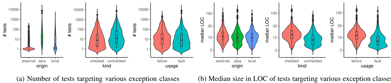
Fig. 4: Violin plots of the analyzed projects’ total number of tests and median size of a test. Each plot groups data according to various characteristics of the exceptions featured in tests: their origin (Java’s standard libraries, external, or local to the project), their kind (checked or unchecked), and their usage (signaling failure or fault). Vertical scales are logarithmic.
