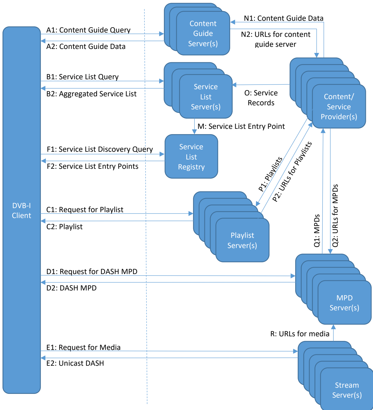
Figure 1: Simplified example DVB-I components and interfaces
