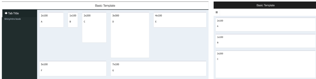
Figure 2.5: An example fluidRow layout of boxes with different widths and heights.
