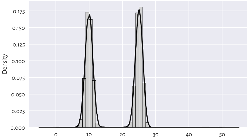
Figure 15.3. Density estimation based on fixed-radius search.
