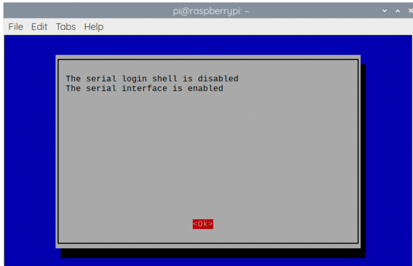
Figure 12. Enabling a serial UART using raspi-config on the Raspberry Pi.
