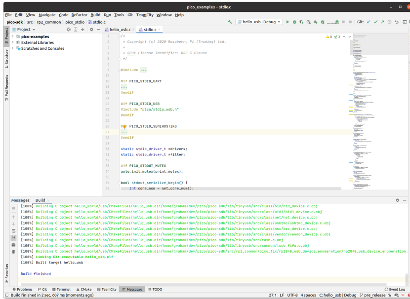
Figure 24. hello_usb successfully built.
