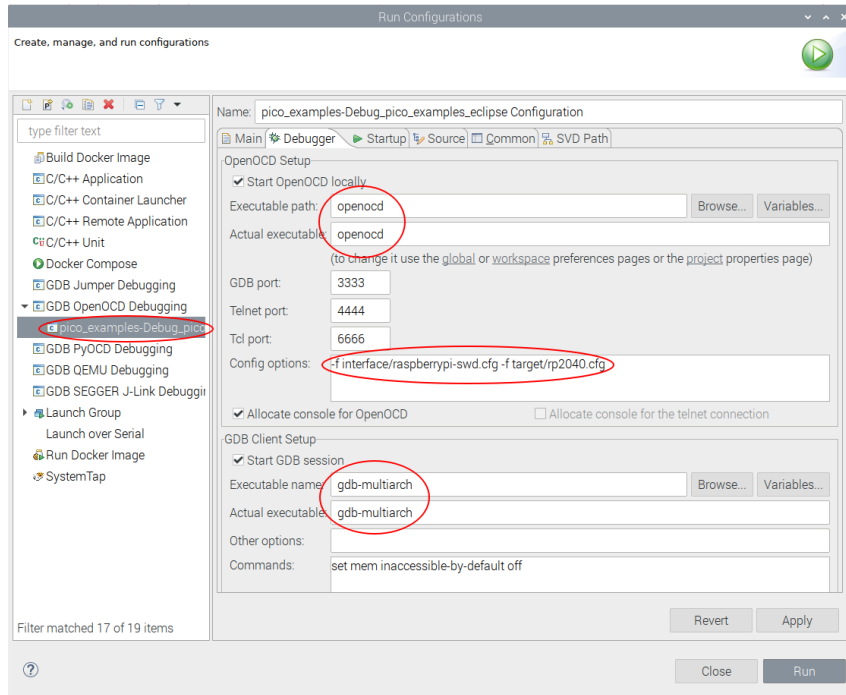
Figure 17. Setting up the Debugger and OpenOCD in Eclipse.
