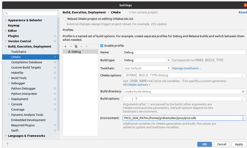
Figure 21. Configuring a CMake profile in CLion.
