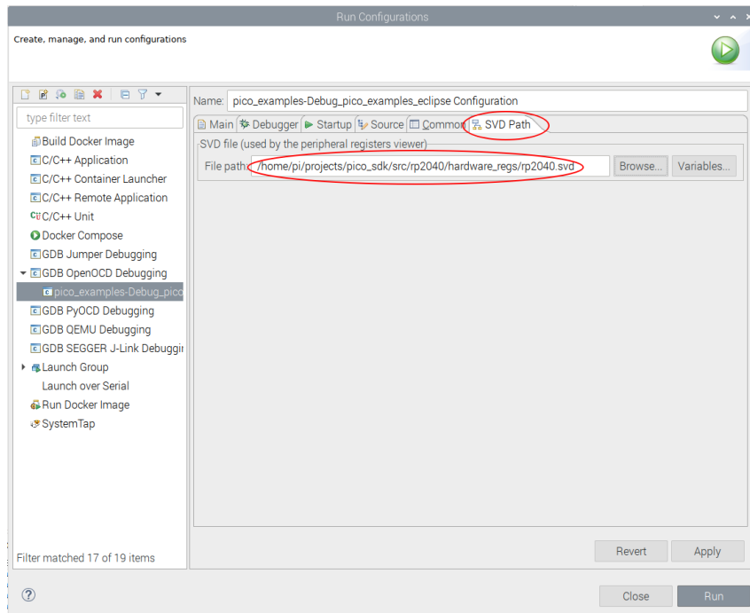
Figure 18. Setting the SVD path in Eclipse.
