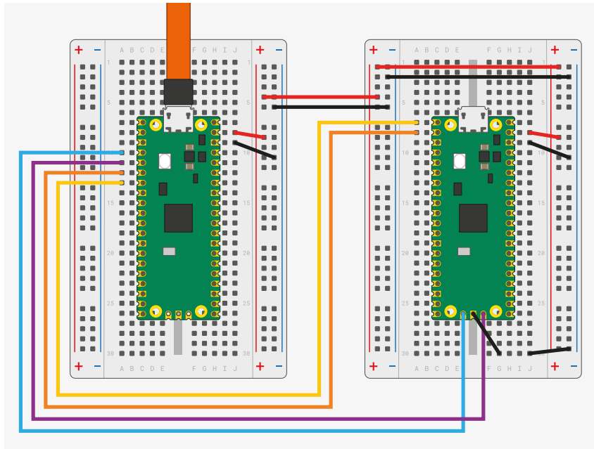
Figure 11. Wiring between Pico A (left) and Pico B (right), configuring Pico A as a debugger.
