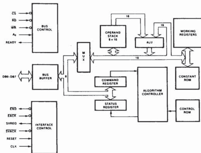
Figure 1. Block Diagram
