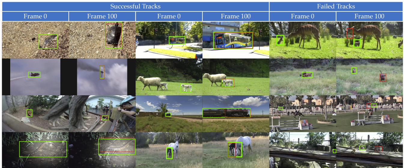
Fig. 7. Qualitative Results: Examples of our tracker on the Imagenet Video [33] dataset. We show the initial frame as well as the 100th frame. Green represents the ground truth box and red represents Re 3 's output. We include challenging examples of scale, appearance, and aspect ratio change as well as occlusion. On the right, we show failures due to latching onto a foreground object, confusion with a similar object, latching onto an occluder, and small or ambiguous initial bounding box.
