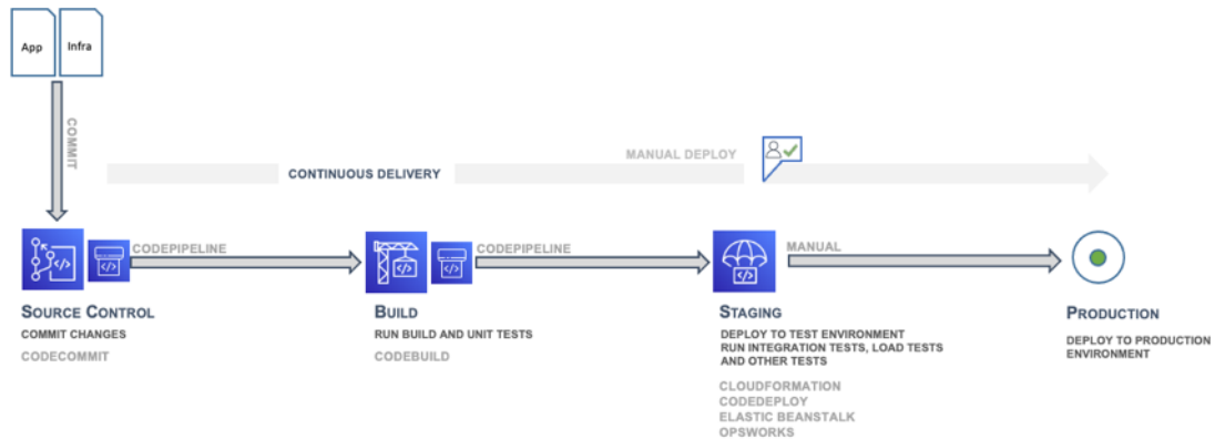
Continuous delivery—staging
