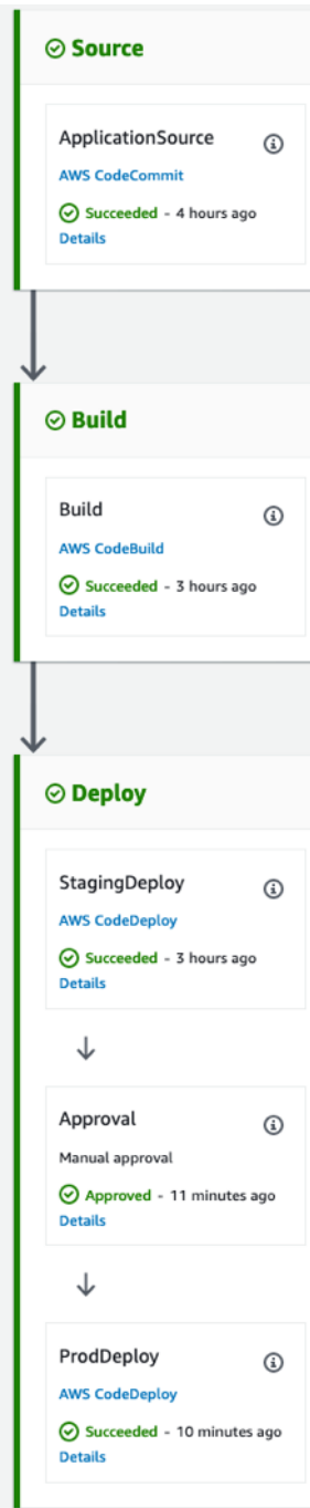
AWS CodePipeline stages
