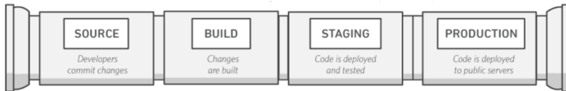
CI/CD pipeline
