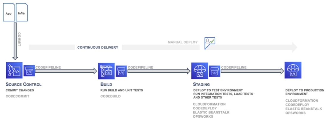
Continuous delivery—production
