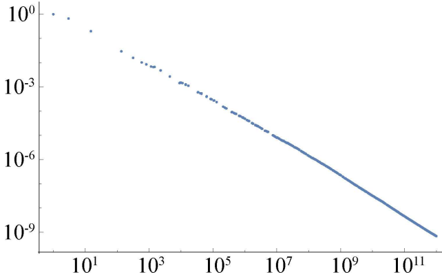
Fig. 1. Density of \mathcal{S} up to k = 10^{12}
