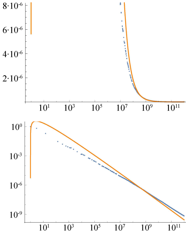
Fig. 2. Density of \mathcal{S} (blue) and A(k) = 10 \log(k)/k (orange) up to k = 10^{12}
