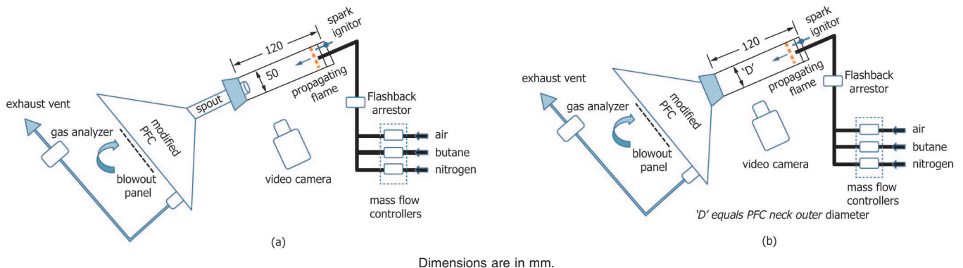
FIG. 1 FMD Effectiveness Test Apparatus (a) With Spout On (b) With Spout Off
