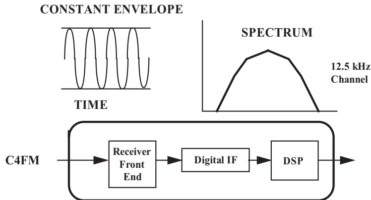
Figure 1-4: C4FM Demodulator
