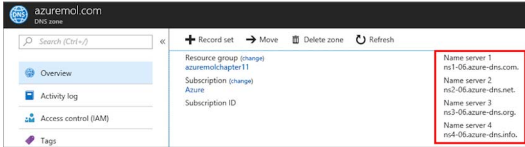
Figure 11.4 You can view the Azure name servers for your DNS zone in the Azure portal, Azure CLI, or Azure PowerShell.
