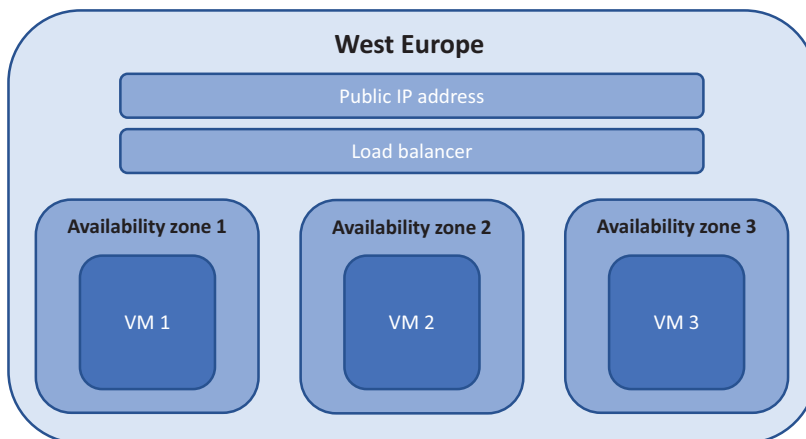
Figure 7.9 An Azure region can contain multiple availability zones: physically isolated datacenters that use independent power, network, and cooling. Azure virtual network resources such as public IP addresses and load balancers can span all zones in a region to provide redundancy for more than just the VMs.
