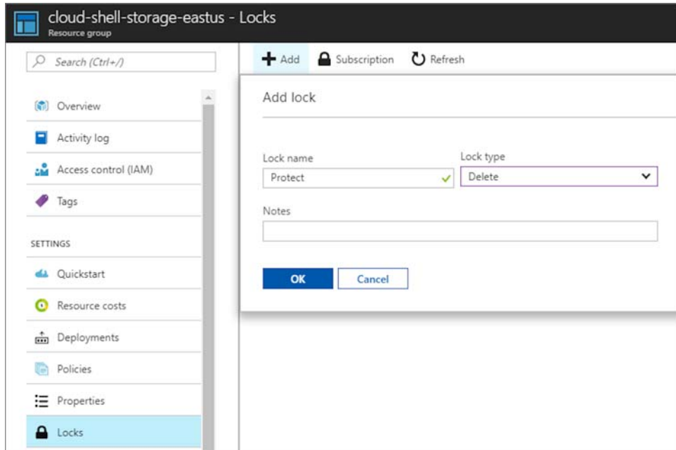
Figure 6.4 Create a resource lock in the Azure portal.
