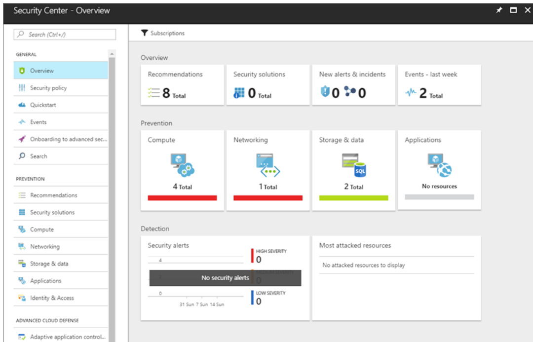
Figure 16.2 The Azure Security Center Overview window provides a list of recommendations, alerts, and events. You can select a core resource type such as Compute or Networking to view a list of security items specific to those resources.
