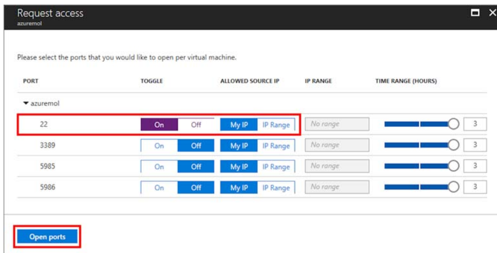
Figure 16.8 When you request access, only the specific ports and source IPs are permitted. The defaults are populated from the settings you provided when you enabled the VM for JIT, but the values can now be changed as needed for each access request.
