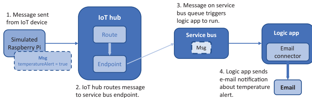
Figure 21.14 The simulated Raspberry Pi device sends a message to the IoT hub every 2 seconds that contains temperature sensor readings. If the temperature is above 30°C, a temperature alert is noted. The IoT hub routes any messages that contain a temperature alert to a service bus queue. Messages on this queue trigger an Azure logic app to run. The logic app is connected to an e-mail provider, such as Outlook or Gmail, and sends an e-mail notification about the temperature warning from the IoT device.
