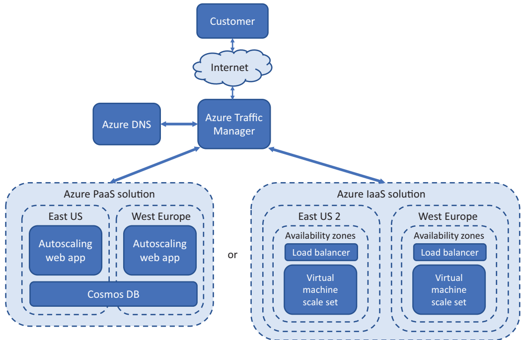
Figure 11.15 After the last few chapters, you should understand how to create highly available IaaS or PaaS applications in Azure. The IaaS solutions can use availability zones, load balancers, and scale sets. The PaaS solutions can use autoscaling web apps and Cosmos DB. Traffic Manager and Azure DNS can route customers to the most appropriate application instance automatically, based on their geographic location.
