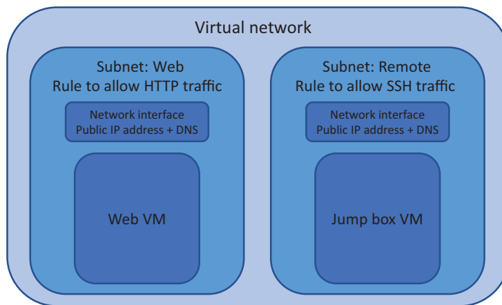
Figure 5.11 (Figure 5.1, repeated.) You're bringing together two subnets, NSGs, rules, network interfaces, and VMs. This is close to a production-ready deployment where one VM runs the web server and is open to public traffic, and another VM in a separate subnet is used for remote connections to the rest of the application environment.
