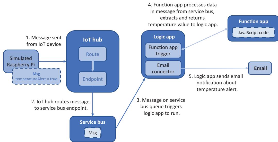
Figure 21.17 As messages are received from the simulated Raspberry Pi device, any messages that contain a temperature alert are routed to the service bus queue endpoint. Messages on the service bus queue trigger a logic app, which passes the message to a function app. A JavaScript function parses the temperature reading and returns it to the logic app, which then sends an e-mail notification that includes the temperature recorded by a sensor on the IoT device.
