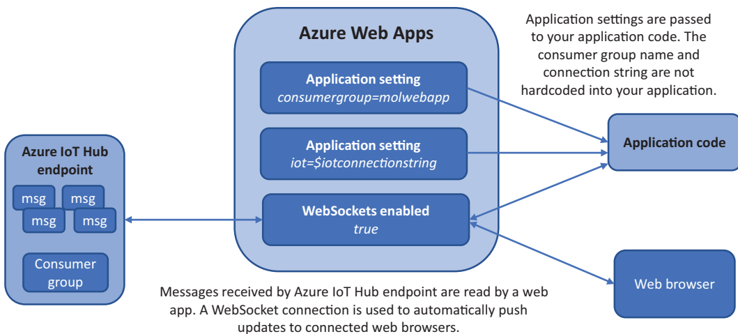
Figure 20.6 To let your web app read the data from your simulated Raspberry Pi IoT device, you create a consumer group in the IoT hub. You then define two application settings for your web app that let you connect to the consumer group. To let your web browser automatically receive the stream of data from the Raspberry Pi as new data is received, you also enable a setting for WebSockets.
