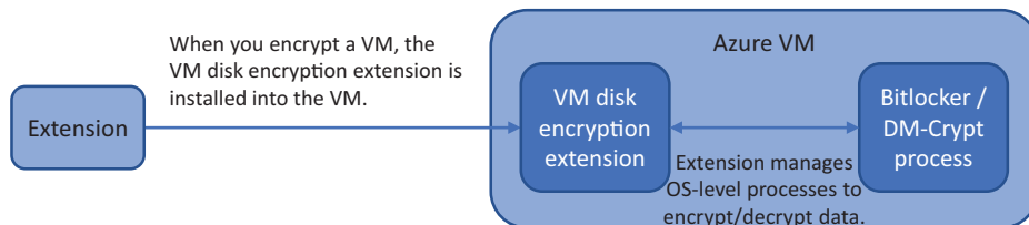
Figure 14.9 When you encrypt a VM, the Azure disk encryption extension is installed. This extension manages the use of BitLocker on Windows VMs or dm-crypt on Linux VMs, to perform the data encryption on your VM. The extension is also used when you query the encryption status for a VM.
