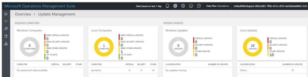
Figure 16.12 The OMS dashboard for Update Management reports the status of configured VMs. As more VMs are added to the service, you can quickly determine how many VMs require patches and how critical the missing patches are in terms of security and compliance. The pie charts show the number of Windows and Linux computers in need of updates, and then how many updates are required for each VM.
