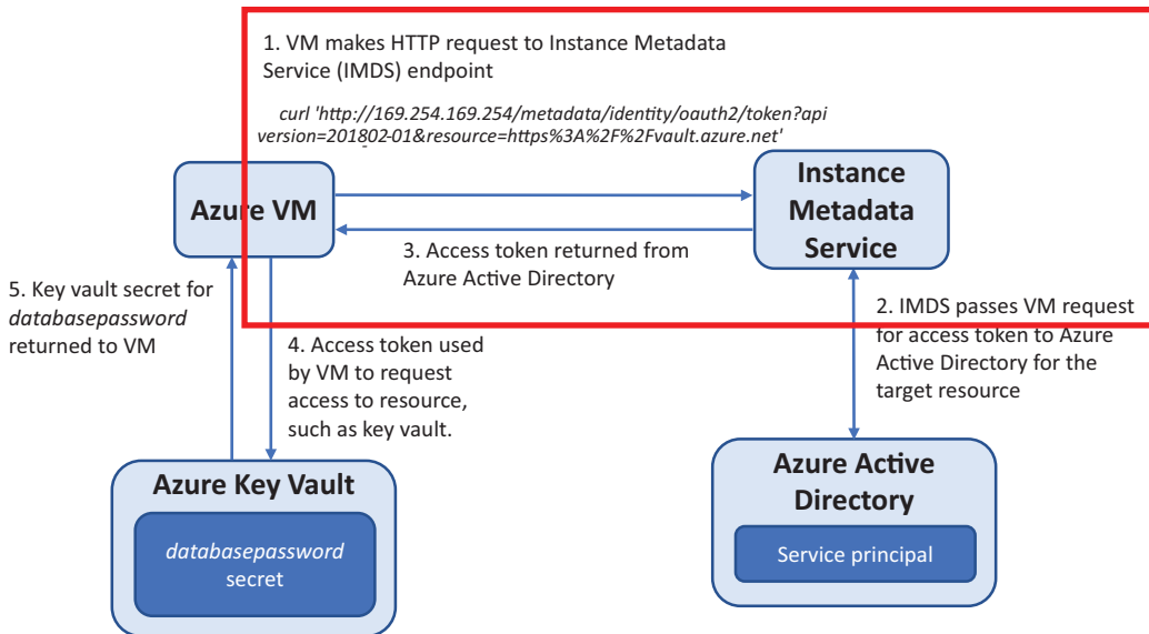
Figure 15.6 The curl request covers the first three steps on this diagram. The curl request is made, the endpoint communicates with AAD, and an access token is issued.
