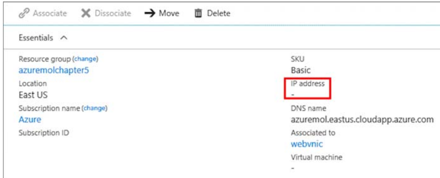
Figure 5.6 The public IP address is now associated with a network interface. With a dynamic assignment, no public IP address is shown until a VM is created and powered on.
