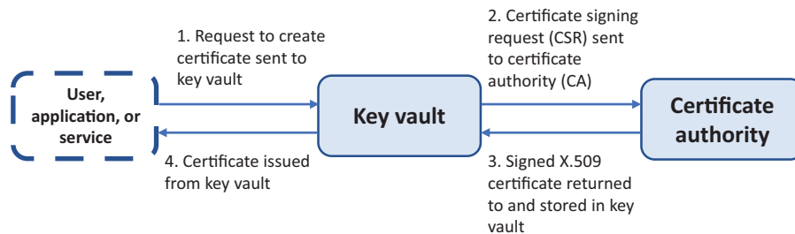
Figure 15.8 A user, application, or service can request a new certificate from a key vault. A certificate signing request (CSR) is sent by the key vault to a certificate authority (CA). This could be an external third-party CA or a trusted internal CA. Azure Key Vault can also act as its own CA to generate self-signed certificates. The CA then issues a signed X.509 certificate, which is stored in the key vault. Finally, the key vault returns the certificate to the original requestor.
