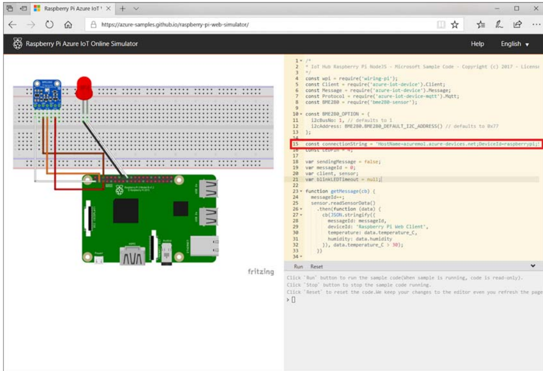
Figure 20.3 Copy and paste the connection string for your Azure IoT device into the Raspberry Pi simulator. The connectionString variable is used to connect to transmit the simulated sensor data to Azure.
