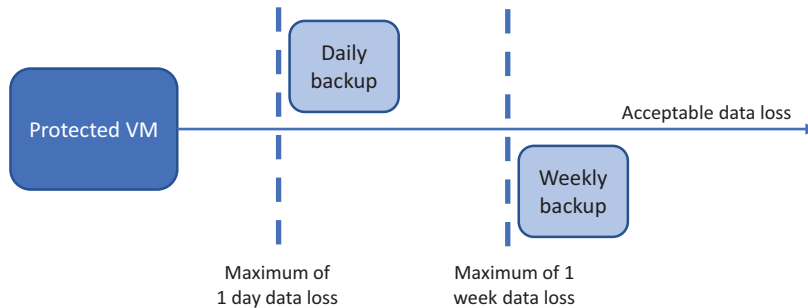
Figure 13.3 The recovery point objective (RPO) defines how much data loss you can sustain for a protected instance. The longer the RPO, the greater the acceptable data loss. An RPO of one day means up to 24 hours of data could be lost, depending on when the data loss occurred in relation to the last backup. An RPO of one week means up to seven days' worth of data could be lost.
