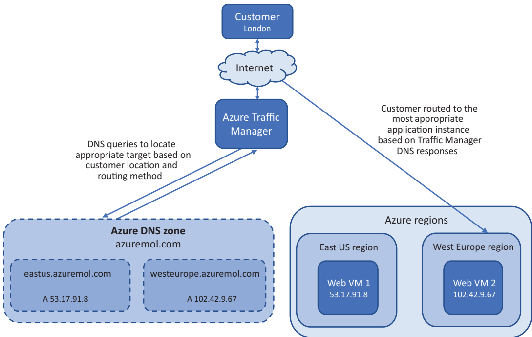
Figure 11.1 In this chapter, we examine how you can create DNS zones in Azure DNS. To minimize latency and improve response times, Traffic Manager can then be used to query DNS and direct customers to their closet application instance.
