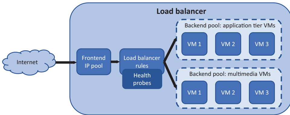
Figure 8.8 One or more backend pools can be created in a load balancer. Each backend pool contains one or more VMs that run the same application component. In this example, one backend pool contains VMs that run the web application tier, and another backend pool contains the VMs that serve multimedia, such as images and video.
