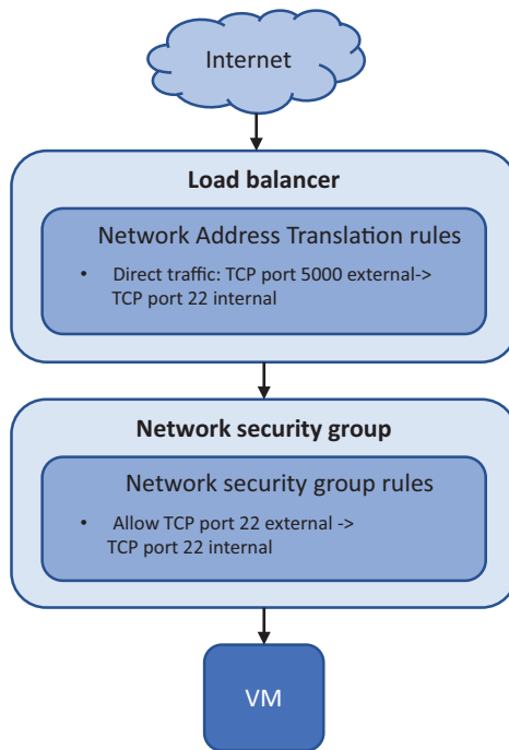
Figure 8.7 Traffic in the load balancer is processed by NAT rules. If a protocol and port match a rule, the traffic is then forwarded to the defined backend VM. No health probes are attached, so the load balancer doesn't check whether the VM is able to respond before it forwards the traffic. The traffic leaves the load balancer and is then processed by NSG rules. If the traffic is permitted, it's passed to the VM.
