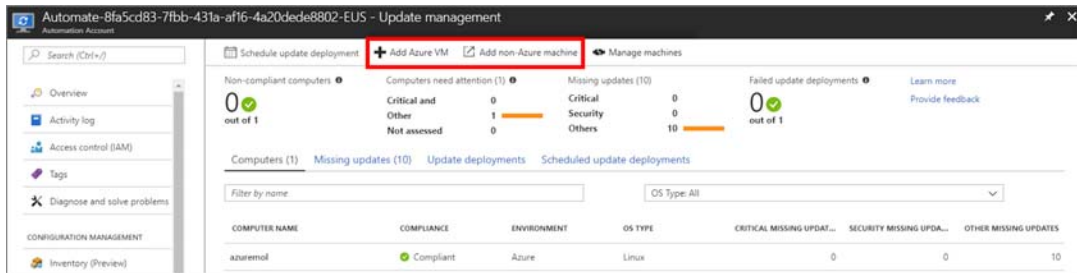
Figure 16.15 In the Azure Automation account, you can manage multiple computers and view the status or apply updates. Both Azure VMs and non-Azure computers can be monitored and controlled by the same Azure Automation account. Behind the scenes, OMS can integrate with other providers to install agents on computers in a hybrid environment. This integration allows a single dashboard and management platform to handle your update needs.
