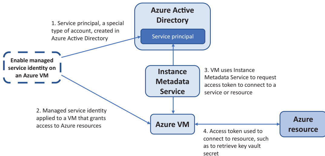
Figure 15.4 When you create a managed service identity for a VM, a service principal is created in Azure Active Directory. This service principal is a special type of account that can be used for resources to authenticate themselves. This VM then uses the Instance Metadata Service endpoint to make requests for access to resources. The endpoint connects to AAD to request access tokens when the VM needs to request data from other services. When an access token is returned, it can be used to request access to Azure resources, such as a key vault.
