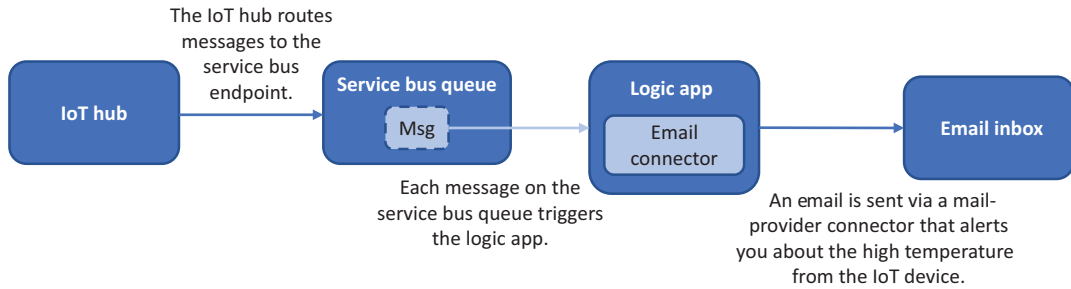
Figure 21.10 Each message received on the service bus queue from the IoT hub triggers the logic app. When the logic app runs, it sends an email notification through a defined mail provider.
