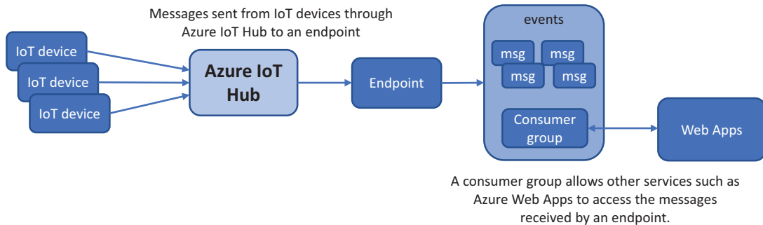
Figure 20.5 Messages are sent from IoT devices to the IoT hub, which then directs the messages to an endpoint. In each endpoint, consumer groups can be created. These consumer groups allow other Azure services to access the device messages, which they otherwise wouldn't have access to. With consumer groups, you don't have to use message queues to allow external applications to read IoT device data.
