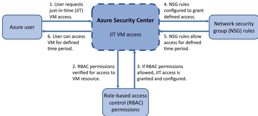
Figure 16.4 With JIT VM access, NSG rules are configured to deny remote connections to a VM. RBAC permissions are used to verify permissions when a user requests access to a VM. These requests are audited, and if the request is granted, the NSG rules are updated to allow traffic from a given IP range, for a defined period of time. The user can access the VM only during this time. Once the time has expired, the NSG rules automatically revert to a deny state.
