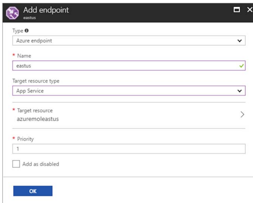
Figure 11.9 Create an endpoint named eastus . The target resource type is App Service. Select the web app you created in East US. With a priority of 1, all traffic is directed to this endpoint, provided the endpoint remains healthy and can serve traffic.
