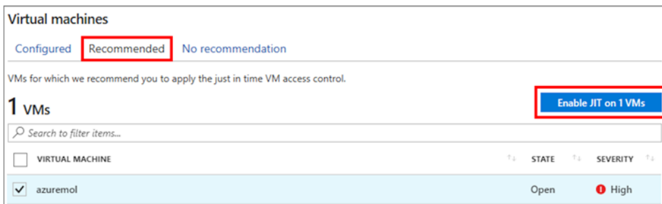
Figure 16.5 Select a VM from the Recommended options, and then choose to Enable JIT on 1 VMs. State currently shows that this VM is Open for all remote access, which flags the severity of the security concern as High.
