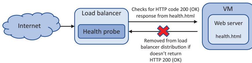
Figure 8.4 A VM that runs a web server and has a custom health.html page remains in the load-balancer traffic distribution provided that the health probe receives an HTTP code 200 (OK) response. If the web server process encounters a problem and can't return requested pages, they're removed from the load-balancer traffic distribution. This provides a more thorough check of the web server state than port-based health probes.
