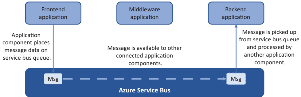
Figure 21.6 Messages are placed in a service bus queue by application components—a frontend app, in this example. Other middleware or backend applications can then pick up these messages and process them as needed. Here, a backend application picks up the message and processes it. Advanced messaging features include guaranteeing the order of messages on the queue, locking messages, timeouts, and relays.
