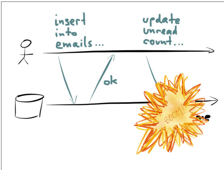
Figure 2-11. One write succeeds; the other write fails. What now?
