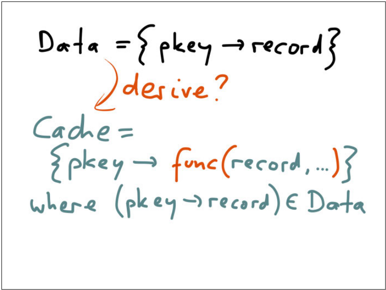
Figure 5-12. Similarly to an index, the contents of a cache are derived from the contents of the database.
