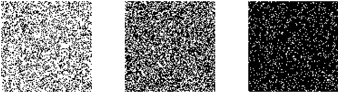
FIG. 11 Three examples of percolation systems on 100 \times 100 square lattices with p = 0.3 , p = p_c = 0.5927\dots and p = 0.9 . The first and last are well below and above the critical point respectively, while the middle example is precisely at it.
