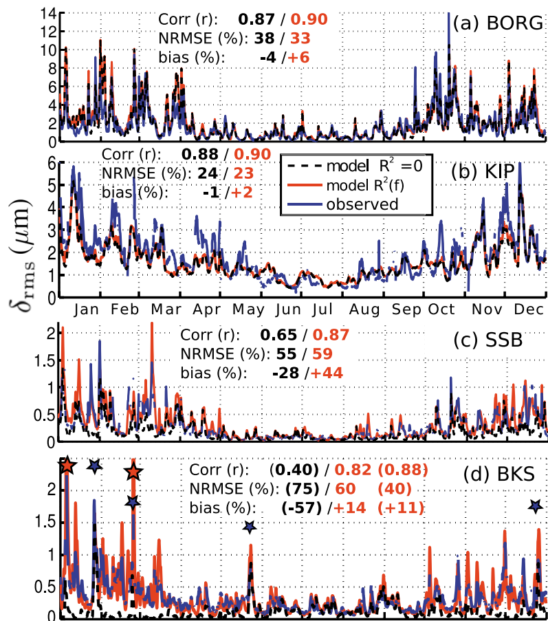
Figure 13. Observed and modeled RMS vertical ground displacement at stations (a) BORG, (b) KIP, (c) SSB, and (d) BKS over the year 2008. The statistics given in each plot quantify the model observation differences, in red for the full model and in black for the model without reflection. These are Pearson’s linear correlation coefficient ( r ), the root mean square error normalized by the root mean square observed value (NRMSE), and the bias normalized by the root mean square observed value. The downward pointing blue stars in the BKS time series mark the times of the largest modeled peaks without reflection, including the 26 January event. The two upward pointing red stars correspond to situations where the model largely overpredicts the observed levels (these two peaks have been clipped). Statistics excluding these two events (less than 1% of the time series) are given in parentheses.
