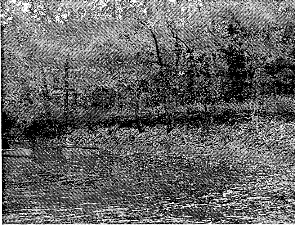
Figure 9. Careful placement of riprap can allow the preservation of mature trees along the banks and avoid impacts associated with their removal
