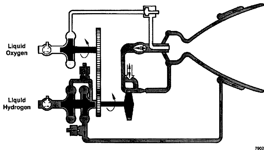
Figure 2 - RL10 Expander Cycle System with Geared LOX Pump
