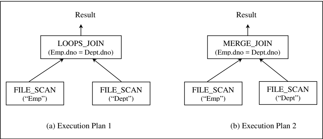
Figure 3. Execution plans
