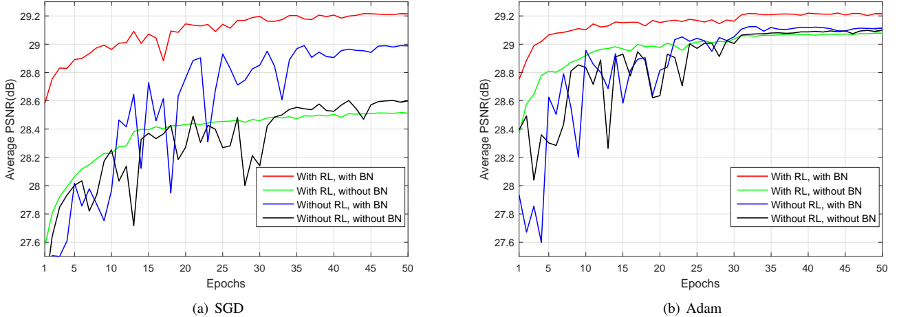
Fig. 2. The Gaussian denoising results of four specific models under two gradient-based optimization algorithms, i.e., (a) SGD, (b) Adam, with respect to epochs. The four specific models are in different combinations of residual learning (RL) and batch normalization (BN) and are trained with noise level 25. The results are evaluated on 68 natural images from Berkeley segmentation dataset.
