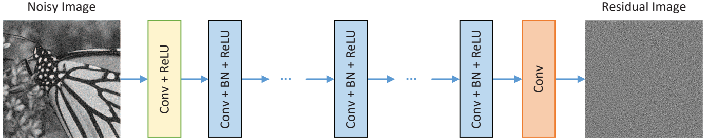
Fig. 1. The architecture of the proposed DnCNN network.
