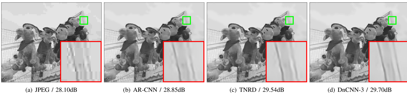
Fig. 12. JPEG image deblocking results of “Carnivaldolls” from LIVE1 dataset with quality factor 10.
