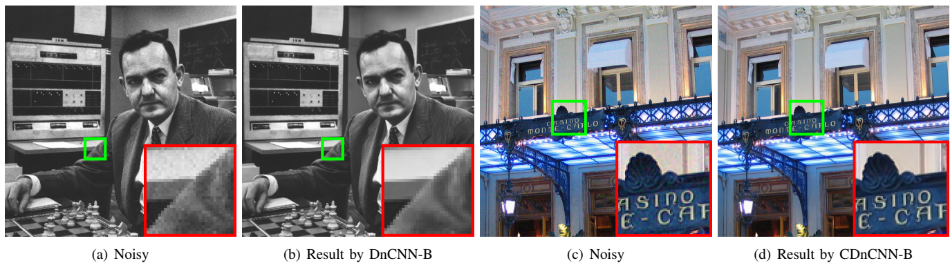
Fig. 8. Gaussian denoising results of two real images by DnCNN-B and CDnCNN-B models, respectively.
