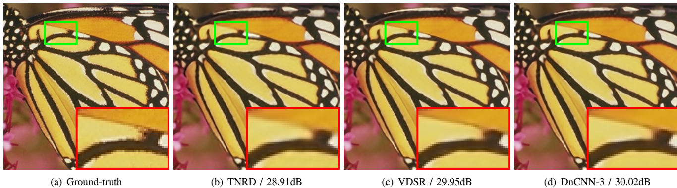
Fig. 10. Single image super-resolution results of “butterfly” from Set5 dataset with upscaling factor 3.
