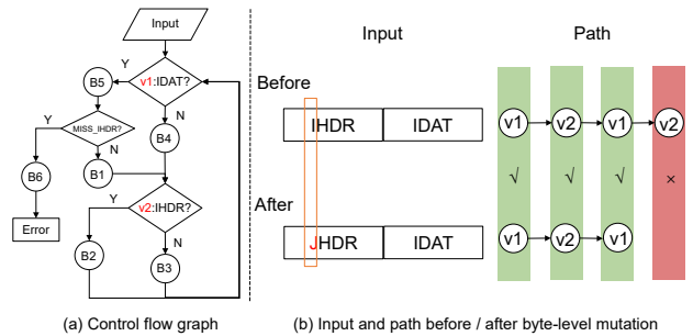
Fig. 2. When execution paths alter after input perturbation, PATA utilizes a matching algorithm to determine which constraint variable occurrence after perturbation matches with a constraint variable occurrence in the original path. Matched pairs are marked with \checkmark in the figure.
