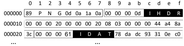
Fig. 1. A sample PNG file. It shows the first two necessary chunks: the image header chunk, IHDR; and the image data chunk, IDAT.
