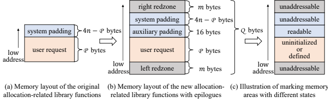
Fig. 2. Memory layout and corresponding accessible states of the allocation-related standard library functions.
