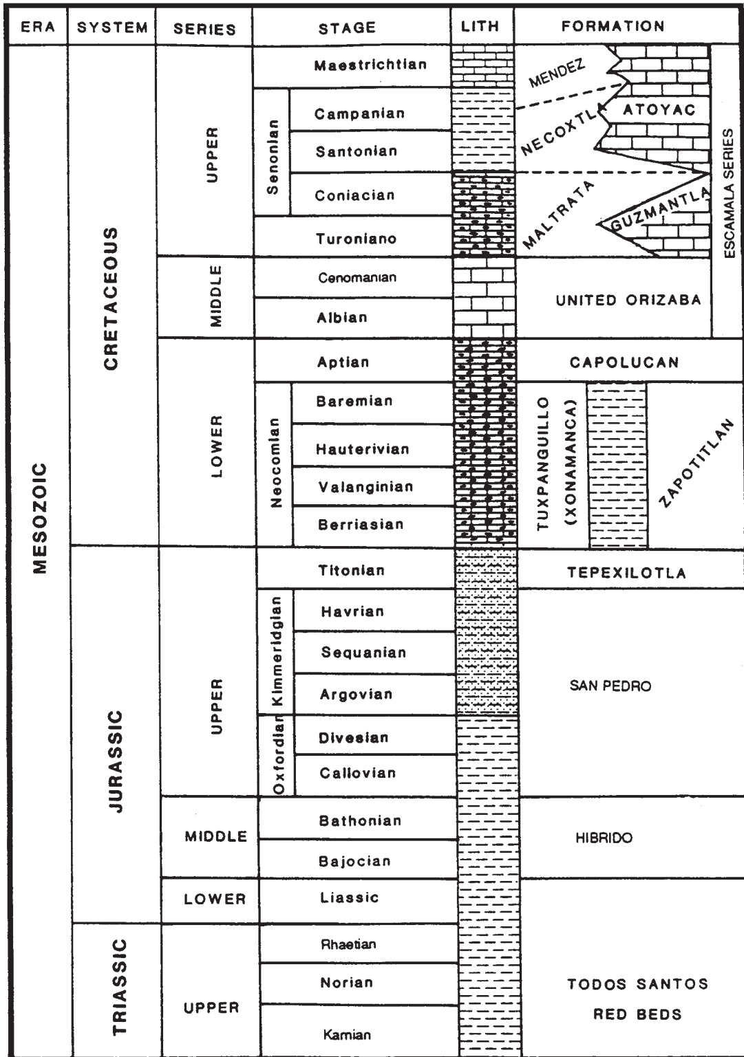
Figure 3.2. Stratigraphic column of the Sierra Juárez. Compiled from Echanove 1963, Viniegra 1965, Moreno 1980, and Ramos 1983.
