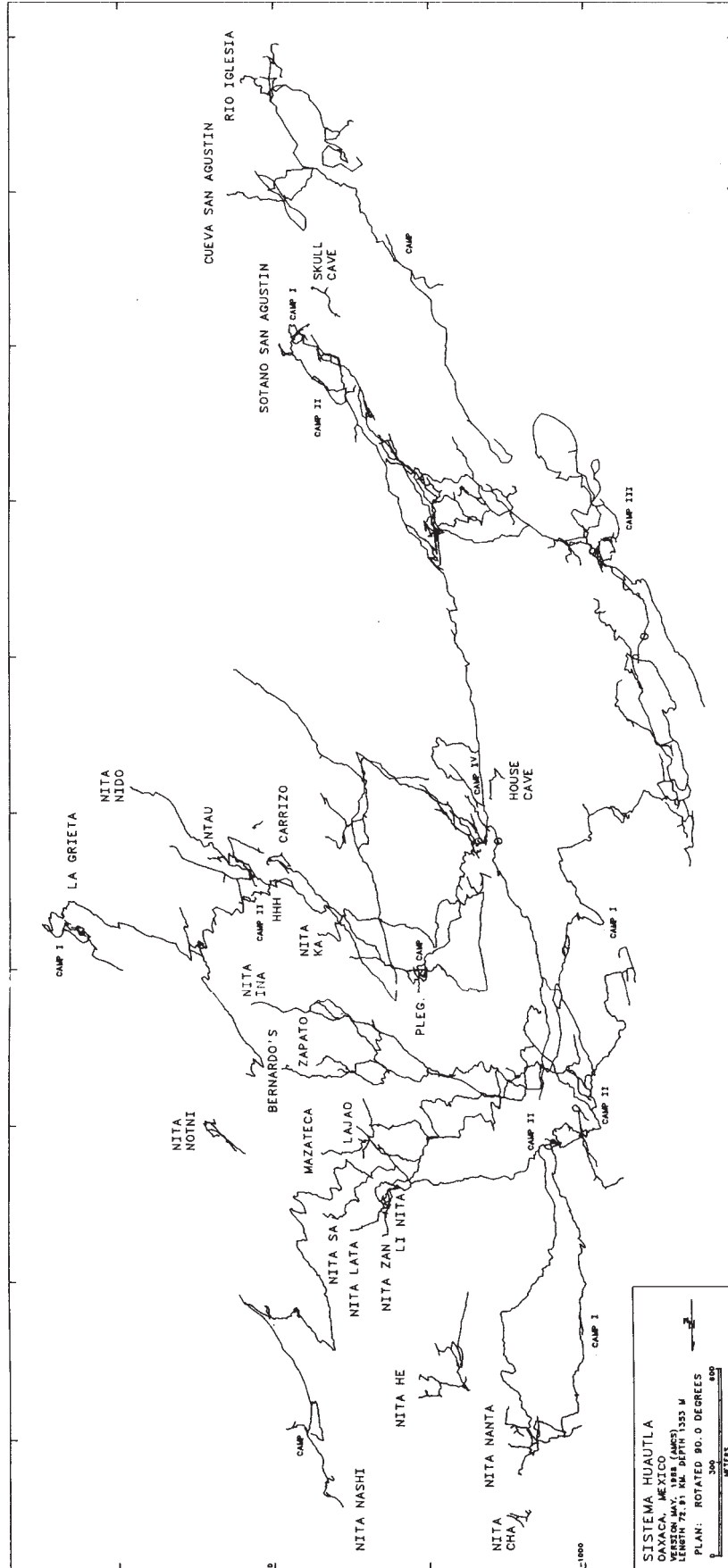
Figure 1.3. Plan view of Sistema Huautla. Source: Smith 1988c.
