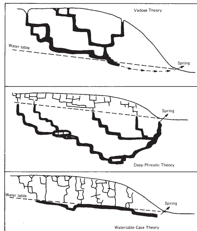
Figure 2.1. Three general models of cave development: vadose theory, deep phreatic theory, and water table cave theory. Source: Ford and Ewers 1978.
