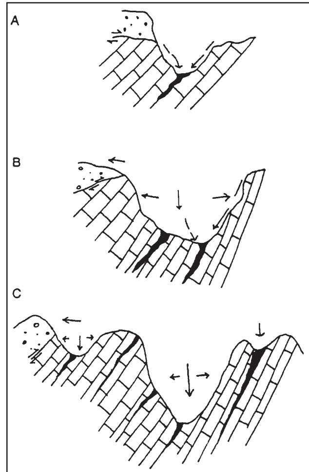
Figure 7.5. Evolution of a dolina in steeply dipping limestone and the corresponding relationship of cave entrances located on ridge tops and cone-karst hills. A. Dolina forms next to allochthonous clastics from allogenic recharge. B. As the clastic cap rock retreats, the dolina enlarges in depth and width. The original drainage outlet is abandoned and stranded higher on the dolina wall, as allogenic recharge drains at the bottom of the dolina through a newly formed conduit. C. Remnant to the retreat of the cap rock are numerous dolinas. Original vadose conduits formed by allogenic recharge are enlarged by autogenic input.
