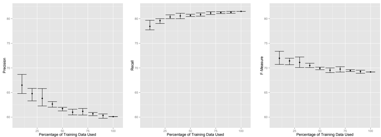
Figure 6: Learning curve on MSM'13 data set.
