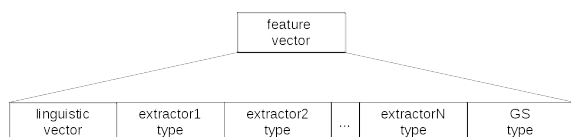
Figure 1: Feature Vector.
