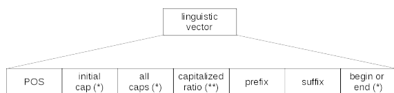
Figure 2: Linguistic Vector.
