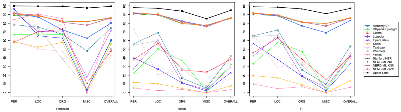
Figure 3: Precision, Recall and F-measure results for individual NERD extractors, Stanford and NERD-ML on CoNLL-2003 Reuters data set for different classes and overall. The black line denotes the upper limit the combined extractors can obtain.
