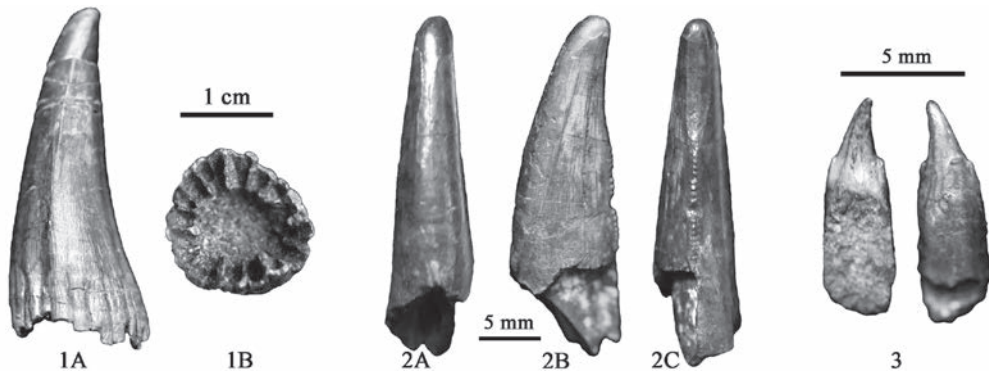
Fig. 5 Teeth of the Jiyuan Fauna
