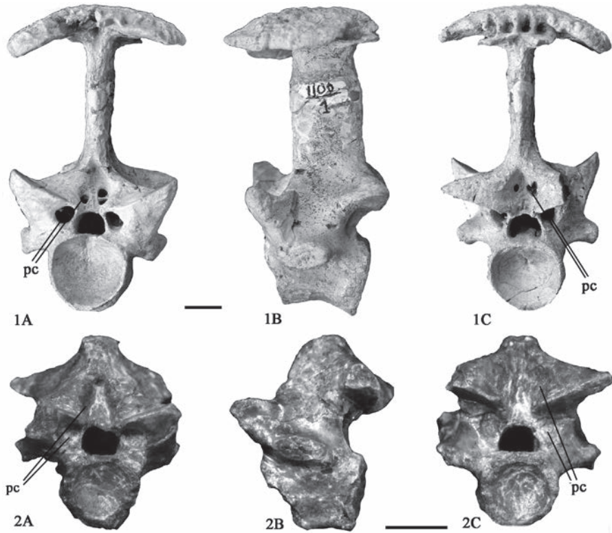
Fig. 4 The vertebrae of Bystrowiana in anterior (A), lateral (B), and posterior (C) views 1. B. permira , PIN 1100/1; 2. B. sinica , HGM 41HIII0445; scale bars equal 1 cm Abbreviation: pc. paraneural canal
