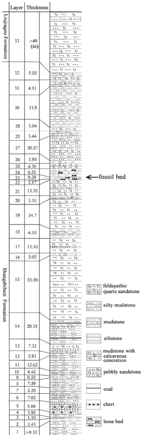
Fig. 2 Lithological column of the 63024 locality
