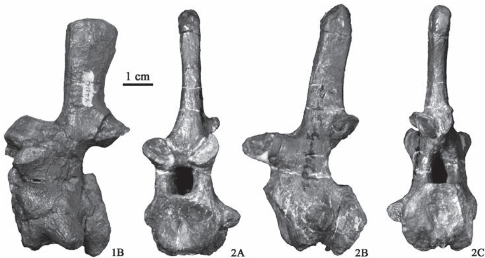
Fig. 6 Two possible therapsid vertebrae in anterior (A), lateral (B), and posterior (C) views 1. IVPP V 4014.2; 2. HGM 41HIII0446
