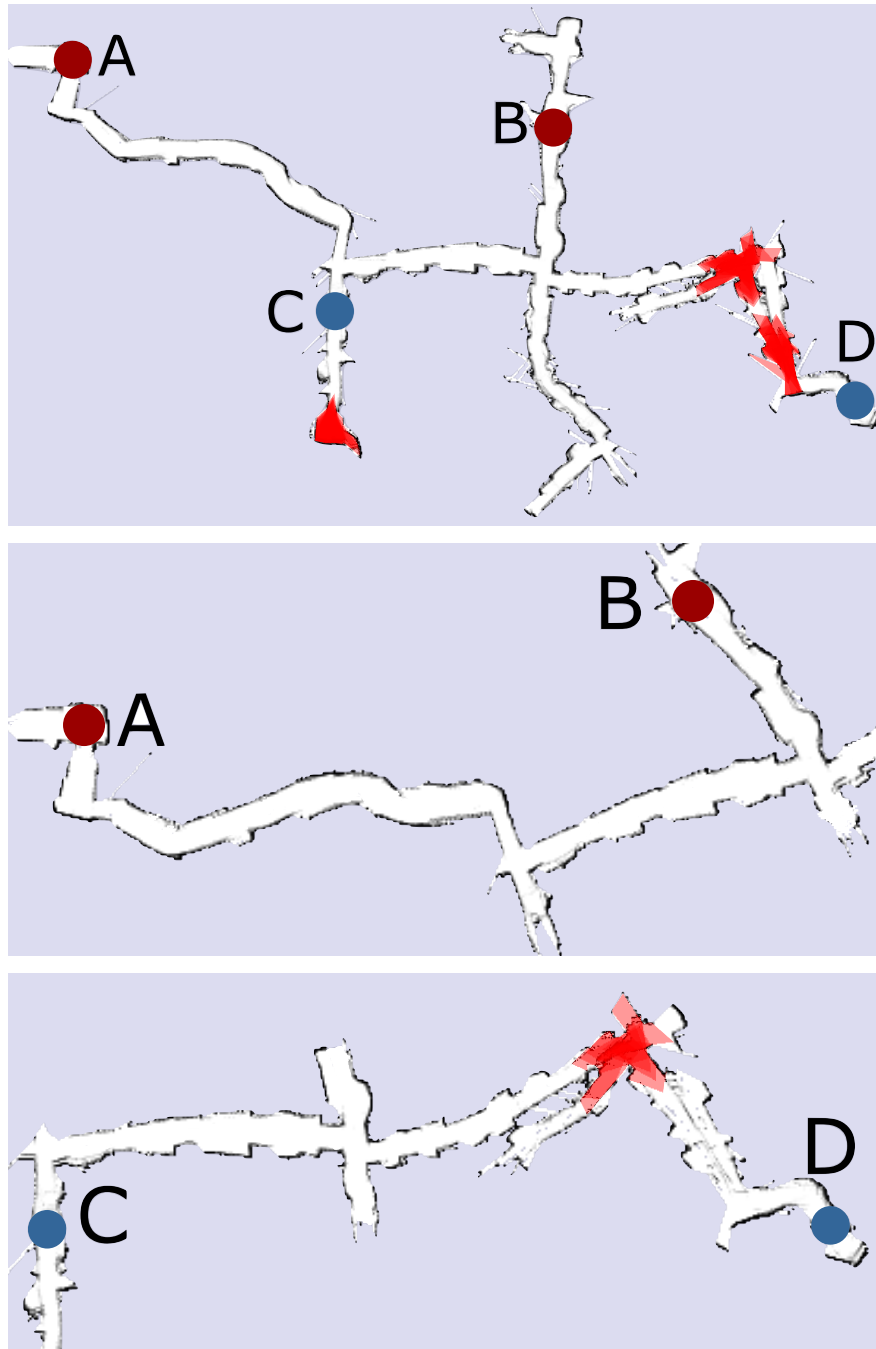
Figure 4.20: Top: a map built so far with the detected inconsistencies (inconsistent scans are shown in red). Middle: image shows a submap that is built using only the scans recorded around the A^* path from A to B computed in the full map. In this example, no inconsistencies are present and none are detected. Bottom: image is constructed in the same way as the middle one, but the A^* path is computed from C to D and here, the map inconsistencies are correctly detected.
