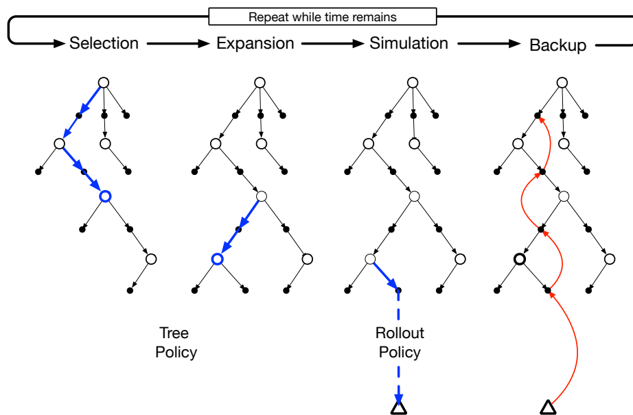
Figure 8.11: Monte Carlo Tree Search. When the environment changes to a new state, MCTS executes as many iterations as possible before an action needs to be selected, incrementally building a tree whose root node represents the current state. Each iteration consists of the four operations Selection , Expansion (though possibly skipped on some iterations), Simulation , and Backup , as explained in the text and illustrated by the bold arrows in the trees. Adapted from Chaslot, Bakkes, Szita, and Spronck (2008).
