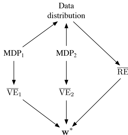
Figure 11.4: Causal relationships among the data distribution, MDPs, and errors for Monte-Carlo objectives. Two different MDPs can produce the same data distribution yet also produce different \overline{\text{VE}} s, proving that the \overline{\text{VE}} objective cannot be determined from data and is not learnable. However, all such \overline{\text{VE}} s must have the same optimal parameter vector, \mathbf{w}^* ! Moreover, this same \mathbf{w}^* can be determined from another objective, the \overline{\text{RE}} , which is uniquely determined from the data distribution. Thus \mathbf{w}^* and the \overline{\text{RE}} are learnable even though the \overline{\text{VE}} s are not.
