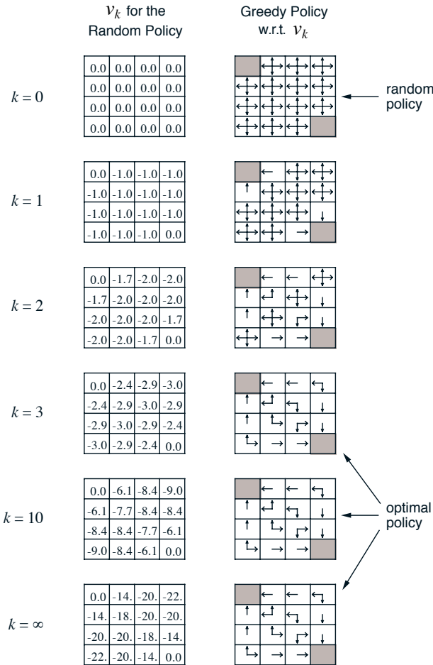
Figure 4.1: Convergence of iterative policy evaluation on a small gridworld. The left column is the sequence of approximations of the state-value function for the random policy (all actions equal). The right column is the sequence of greedy policies corresponding to the value function estimates (arrows are shown for all actions achieving the maximum). The last policy is guaranteed only to be an improvement over the random policy, but in this case it, and all policies after the third iteration, are optimal.
