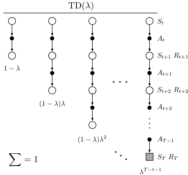
Figure 12.1: The update digram for TD(\lambda) . If \lambda = 0 , then the overall update reduces to its first component, the one-step TD update, whereas if \lambda = 1 , then the overall update reduces to its last component, the Monte Carlo update.
