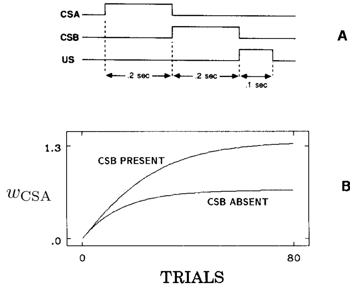
Figure 14.2: Facilitation of a remote association by an intervening stimulus in the TD model. Top: temporal relationships among stimuli within a trial. Bottom: behavior over trials of CSA’s associative strength when CSA is presented in a serial compound as shown in the top panel, and when presented in an identical temporal relationship to the US, only without CSB. Adapted from Sutton and Barto (1990).
