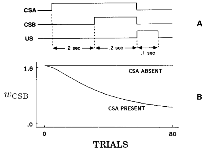
Figure 14.4: Temporal primacy overriding blocking in the TD model. Top: temporal relationships between stimuli. Bottom: behavior over trials of CSB’s associative strength when CSB is presented with and without CSA. The only difference between this simulation and that shown in Figure 14.3 was that here CSB started out fully conditioned—CSB’s associative strength was initially set to 1.653, the final level reached when CSB was presented alone for 80 trials, as in the “CSA-absent” case in Figure 14.3. Adapted from Sutton and Barto (1990).
