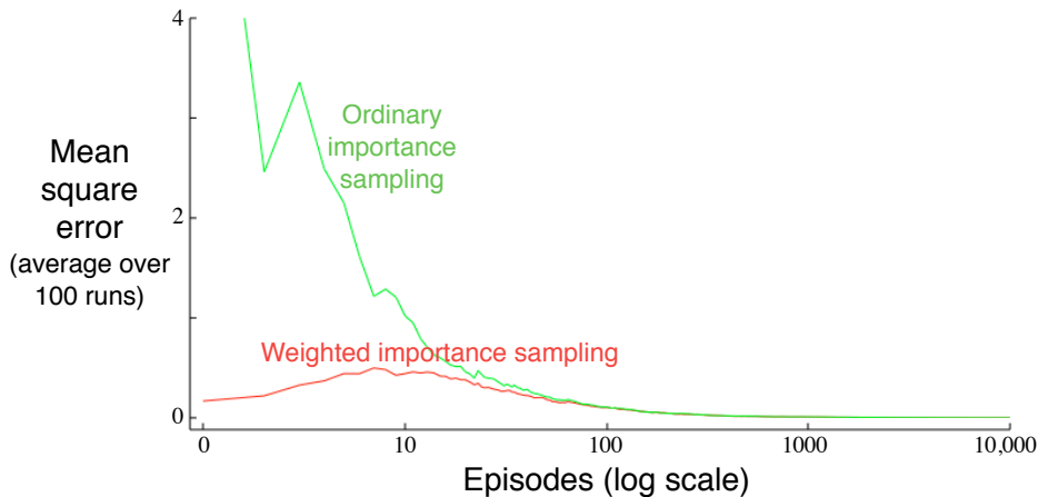
Figure 5.3: Weighted importance sampling produces lower error estimates of the value of a single blackjack state from off-policy episodes (see Example 5.4). ■
