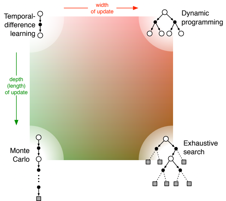
Figure 8.12: A slice through the space of reinforcement learning methods, highlighting the two of the most important dimensions explored in Part I of this book: the depth and width of the updates.
