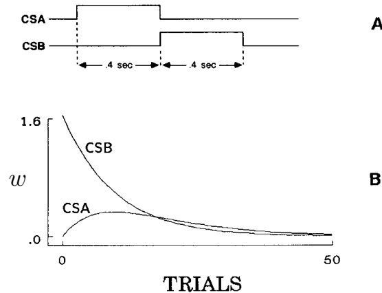
Figure 14.5: Second-order conditioning with the TD model. Top: temporal relationships between stimuli. Bottom: behavior of the associative strengths associated with CSA and CSB over trials. The second stimulus, CSB, has an initial associative strength of 1.653 at the beginning of the simulation. Adapted from Sutton and Barto (1990).
