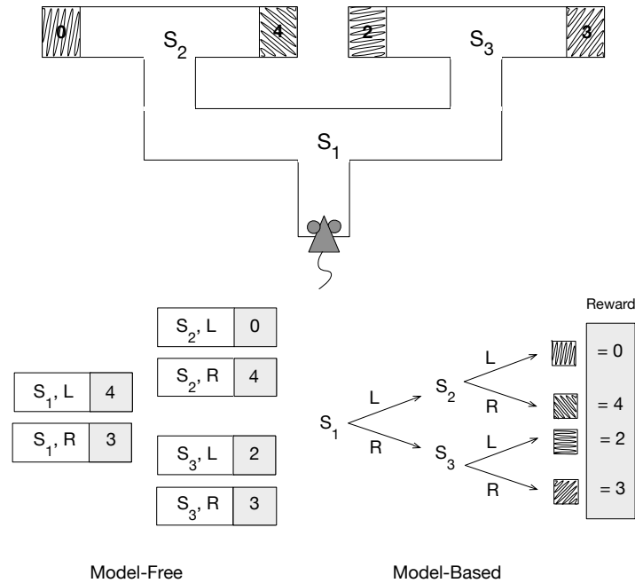
Figure 14.8: Model-based and model-free strategies to solve a hypothetical sequential action-selection problem. Top: a rat navigates a maze with distinctive goal boxes, each associated with a reward having the value shown. Lower left: a model-free strategy relies on stored action values for all the state-action pairs obtained over many learning trials. To make decisions the rat just has to select at each state the action with the largest action value for that state. Lower right: in a model-based strategy, the rat learns an environment model, consisting of knowledge of state-action-next-state transitions and a reward model consisting of knowledge of the reward associated with each distinctive goal box. The rat can decide which way to turn at each state by using the model to simulate sequences of action choices to find a path yielding the highest return. Adapted from Trends in Cognitive Science , volume 10, number 8, Y. Niv, D. Joel, and P. Dayan, A Normative Perspective on Motivation, p. 376, 2006, with permission from Elsevier.
