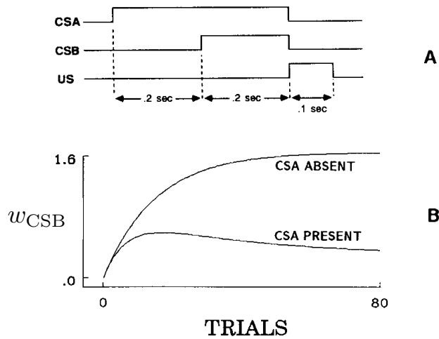
Figure 14.3: The Egger-Miller, or primacy, effect in the TD model. Top: temporal relationships among stimuli within a trial. Bottom: behavior over trials of CSB’s associative strength when CSB is presented with and without CSA. Adapted from Sutton and Barto (1990).
