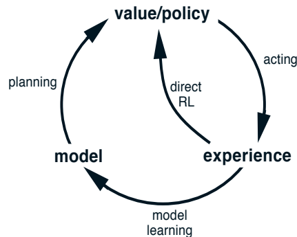
Figure 8.1: Relationships among learning, planning, and acting.
