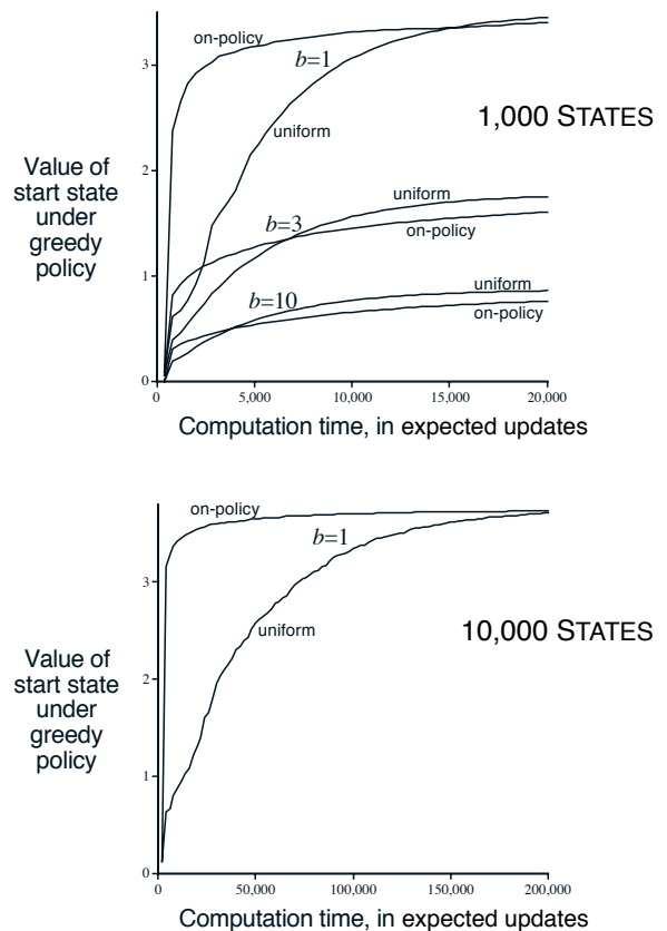
Figure 8.9: Relative efficiency of updates distributed uniformly across the state space versus focused on simulated on-policy trajectories, each starting in the same state. Results are for randomly generated tasks of two sizes and various branching factors, b .
