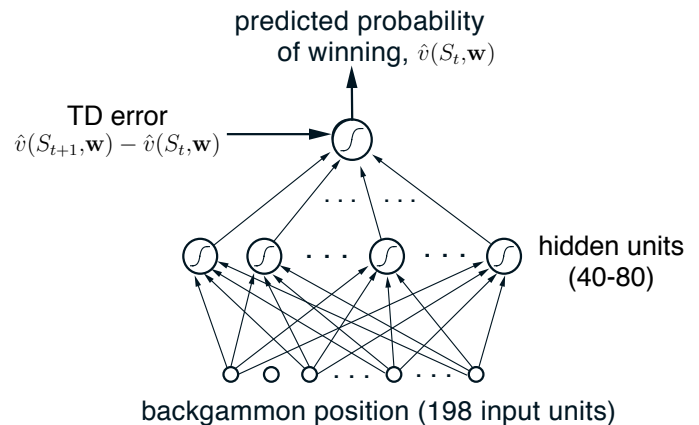
Figure 16.1: The TD-Gammon neural network
