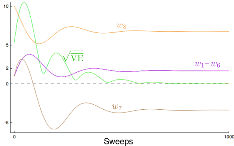
Figure 11.7: The behavior of the one-step emphatic-TD algorithm in expectation on Baird’s counterexample. The step size was \alpha = 0.03 .
