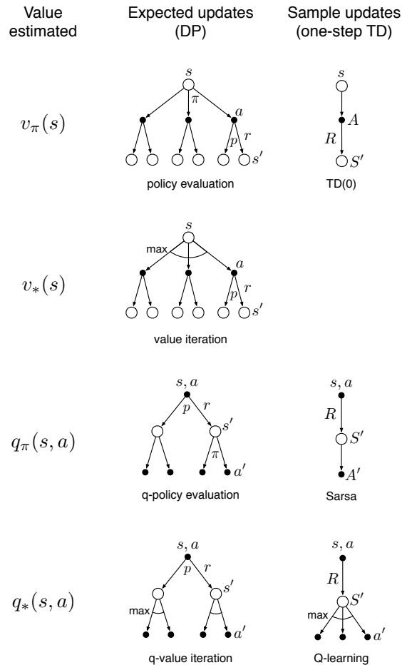
Figure 8.7: Backup diagrams for all the one-step updates considered in this book.
