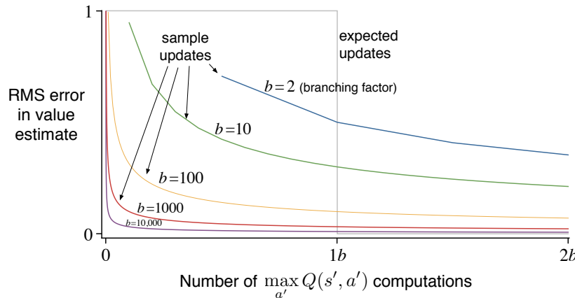
Figure 8.8: Comparison of efficiency of expected and sample updates.
