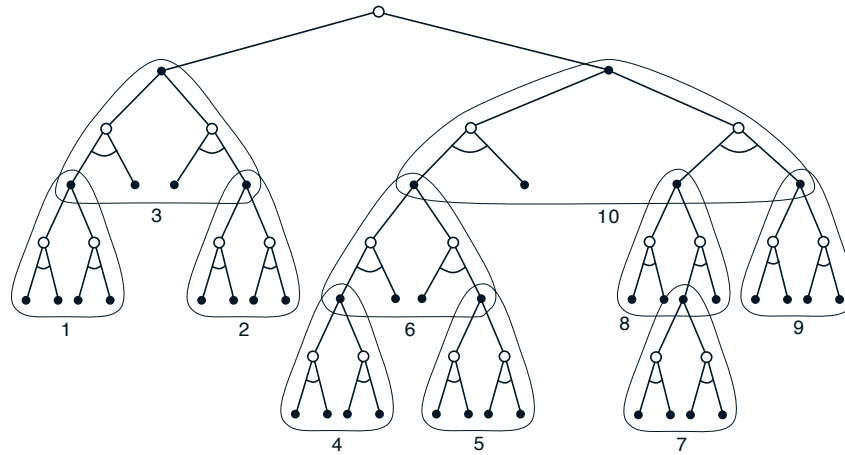
Figure 8.10: Heuristic search can be implemented as a sequence of one-step updates (shown here outlined) backing up values from the leaf nodes toward the root. The ordering shown here is for a selective depth-first search.
