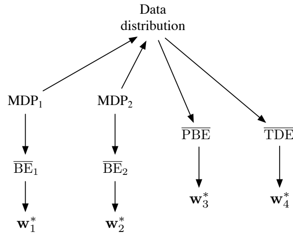
Figure 11.5: Causal relationships among the data distribution, MDPs, and errors for bootstrapping objectives. Two different MDPs can produce the same data distribution yet also produce different \overline{\text{BE}} s and have different minimizing parameter vectors; these are not learnable from the data distribution. The \overline{\text{PBE}} and \overline{\text{TDE}} objectives and their (different) minima can be directly determined from data and thus are learnable.
