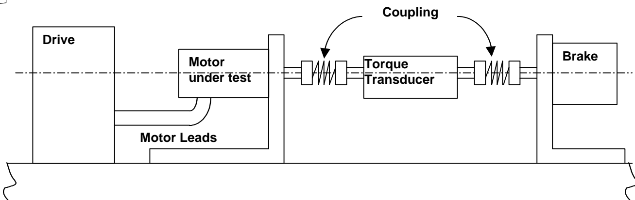
Figure 42 — Typical pull-out torque test set-up (magnetic particle brake dynamometer shown)
