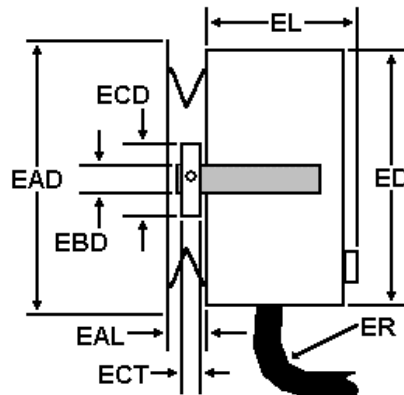
Figure 98 — Format for presenting mounting requirements for through hollow shaft encoders
