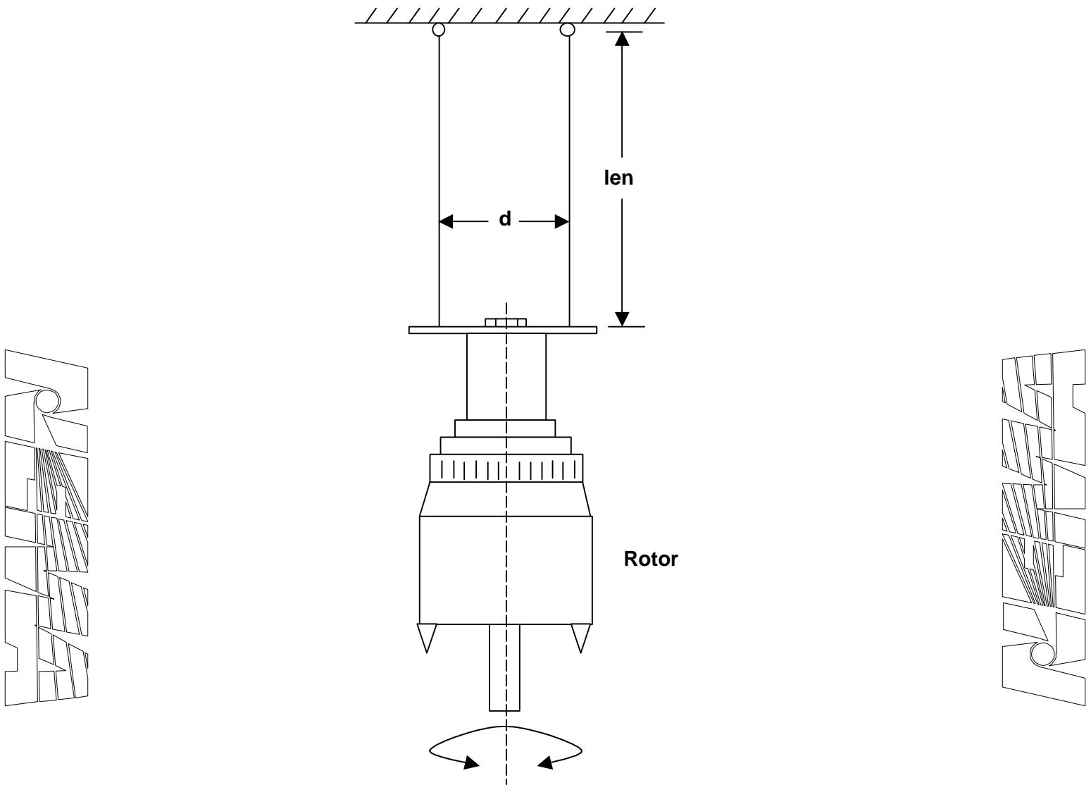
Figure 29 — Moment of inertia wK^2 test: double wire hanging method
