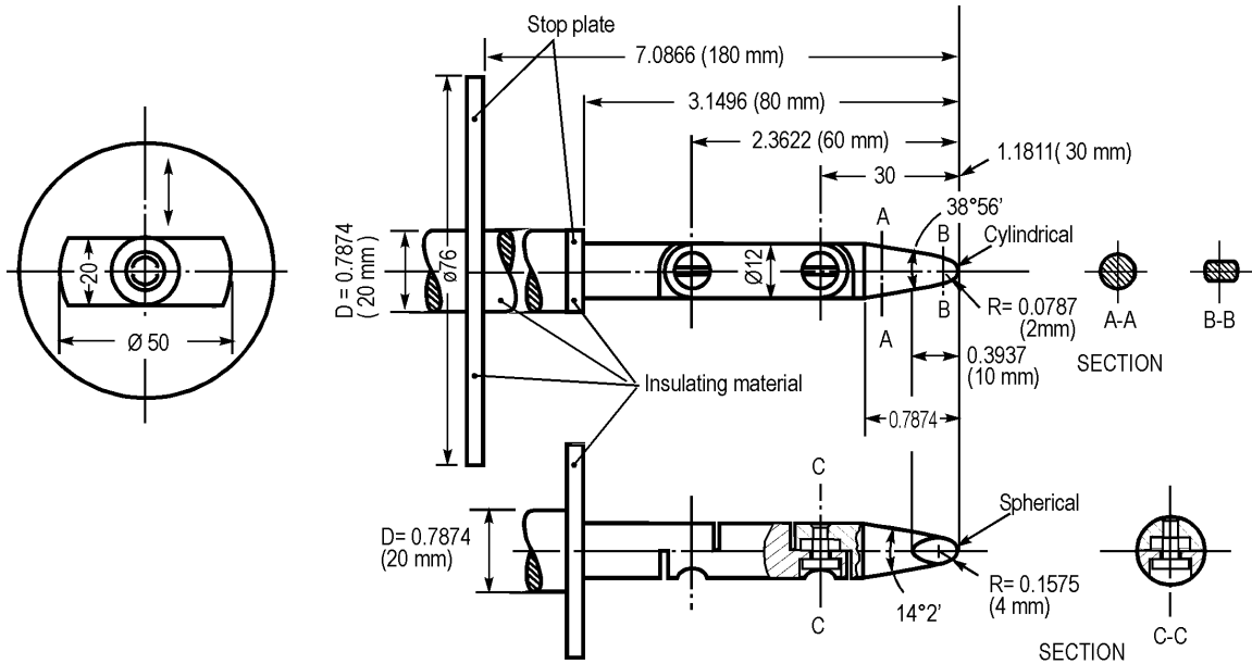
Figure 27 — Articulated probe
