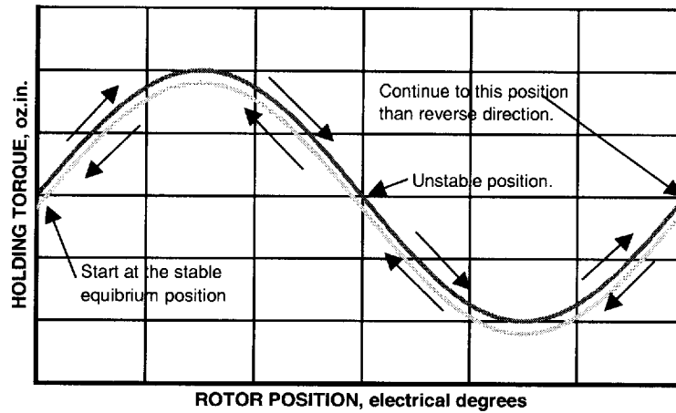
Figure 51 — Desired data points of holding torque measurement
