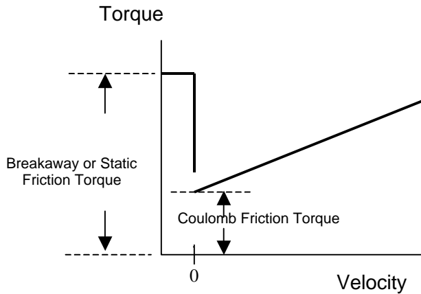
Figure 1 — Friction torque
