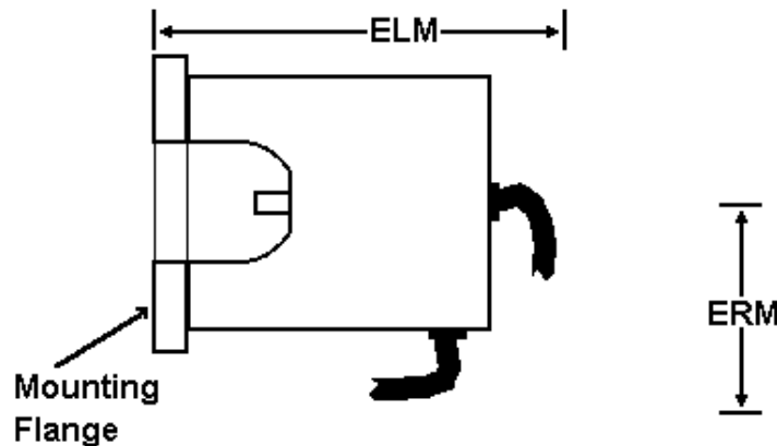
Figure 93 — Format for presenting space requirements for a C-Face encoder with a connector configuration
