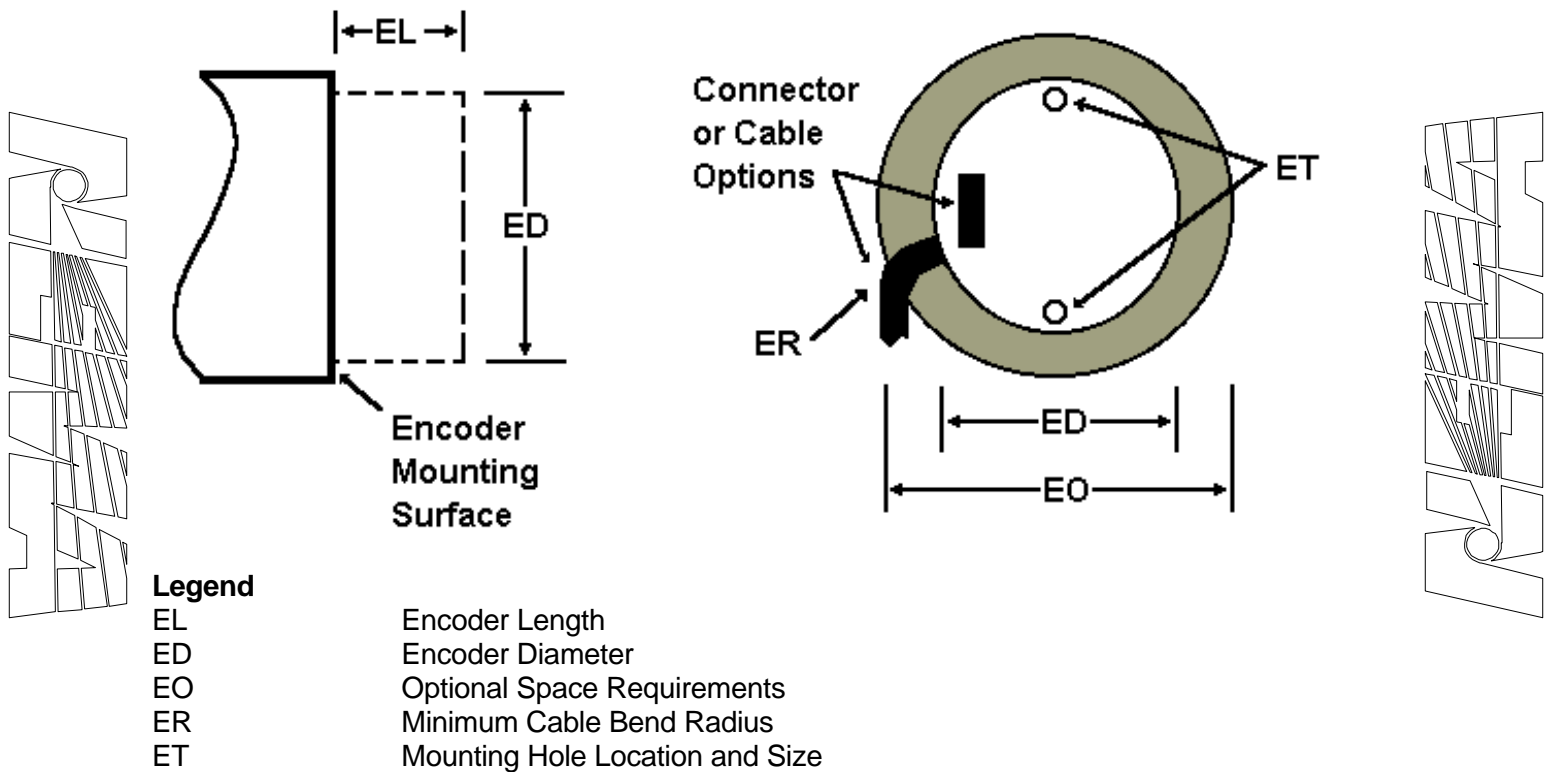
Figure 99 — Format for presenting space requirements for non-commutating bearingless encoders
