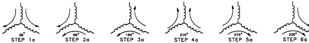
Figure 57 — Additional current paths for 12-step circuitry
