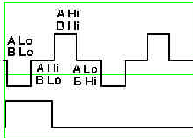
Figure 81 — Gated index with channel B low (180°)
