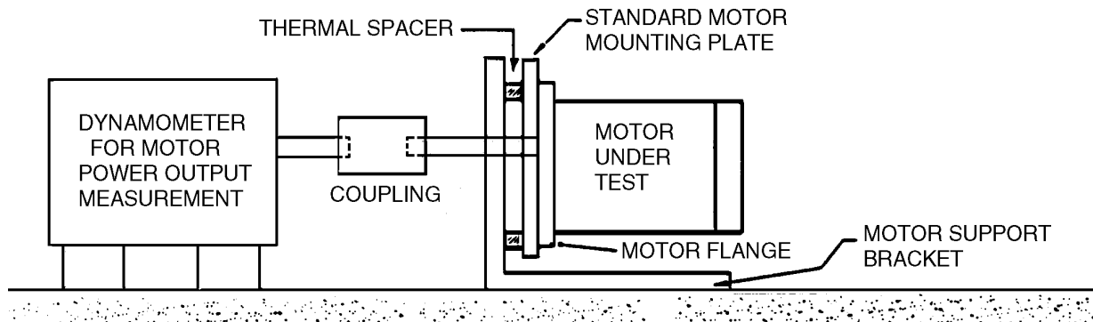
Figure 32 — Flange mounted motor test configuration
