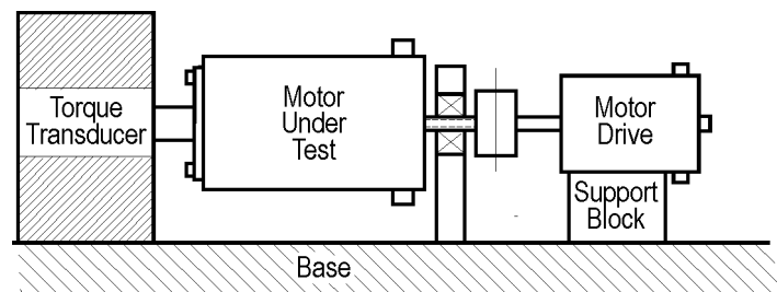
Figure 36 — Viscous Damping test layout
