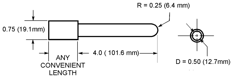
Figure 26 — Probe for film-coated wire
