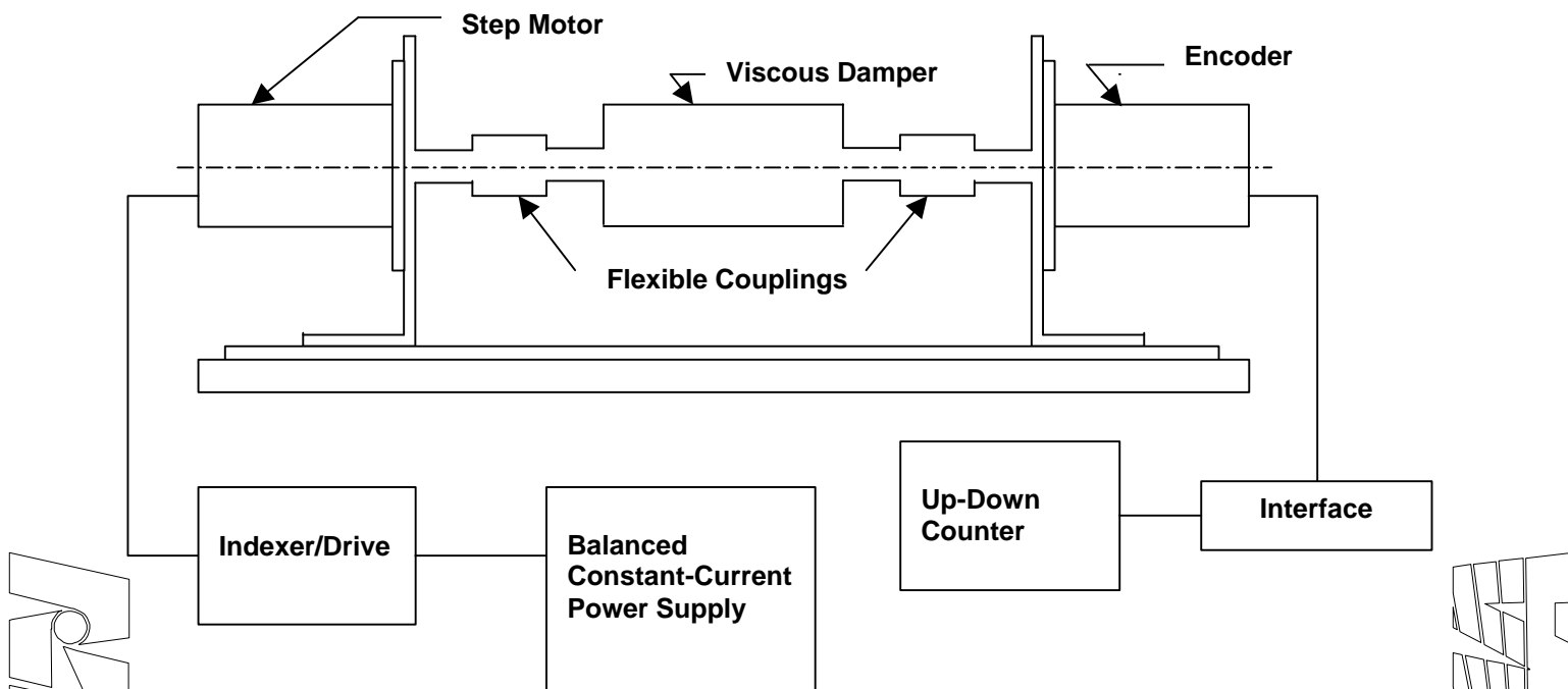
Figure 47— Test set-up for step accuracy
