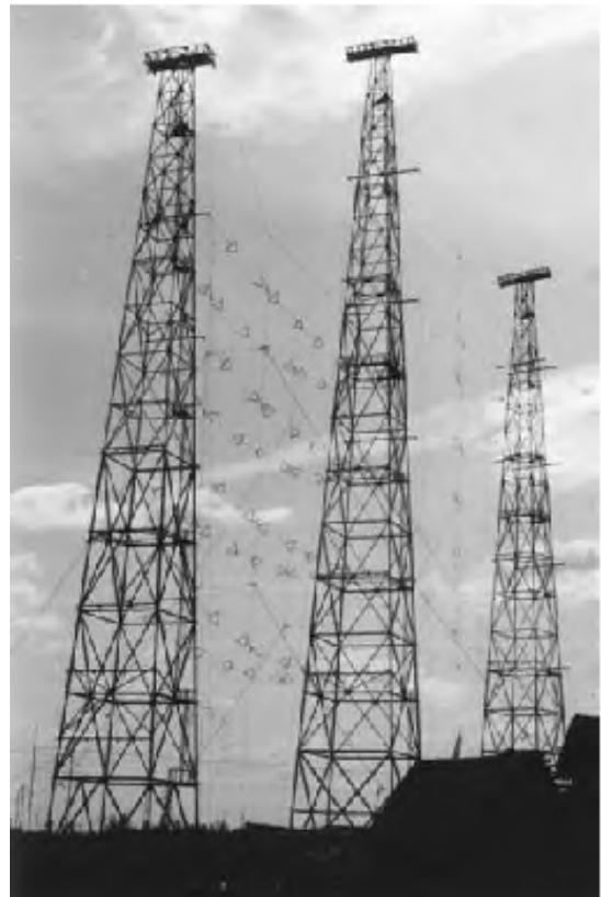
Vertical curtain array SW antennas, used for the long-distance sky wave jamming
