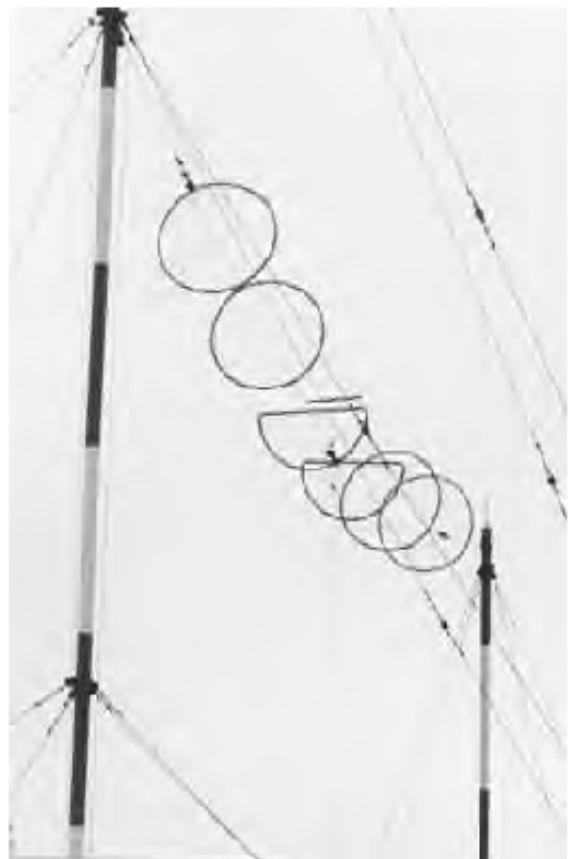
Standard multi-wire broadband "VGDSH" type dipole, used for ground wave jamming in the USSR
