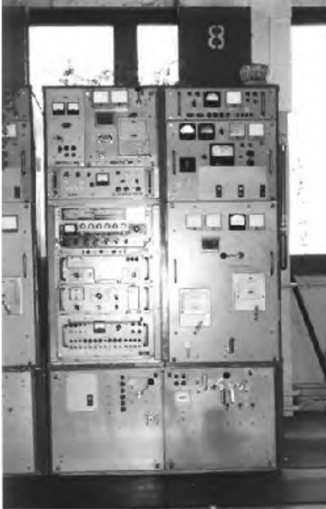
2.5/5 kW SW communications radio transmitters "Viaz-M2" (USSR), used at the local radio jamming stations in the late 70's and 80's.
