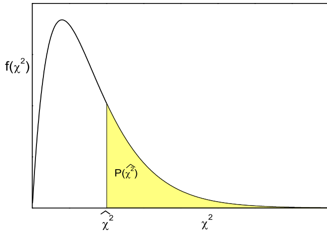
Fig. 10.6. P-value for the obseration \widehat{\chi^2} .
