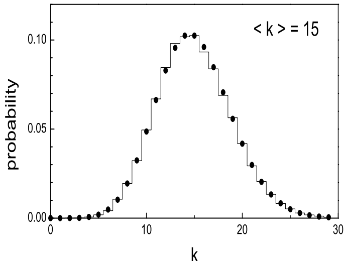
Fig. 3.17. Comparison of a Poisson distribution (histogram) with a scaled distribution of weighted events (dots). The weights are uniformly distributed between zero and one.
