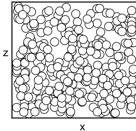
Fig. 5.9. Solid sheres in a box. The plot is a projection onto the x-z plane.
