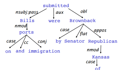
Figure 1: Dependency tree for the sentence "Bills on ports and immigration were submitted by Senator Brownback, Republican of Kansas"
