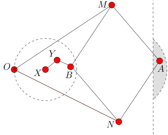
(b) Modified Peaucellier inversor.
