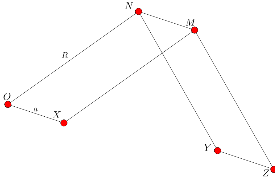
Figure 3-6: Kempe's translator.
