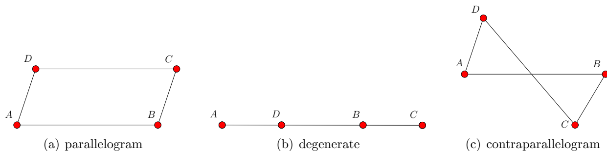
Figure 3-1: The various configurations of a rectangle linkage.
