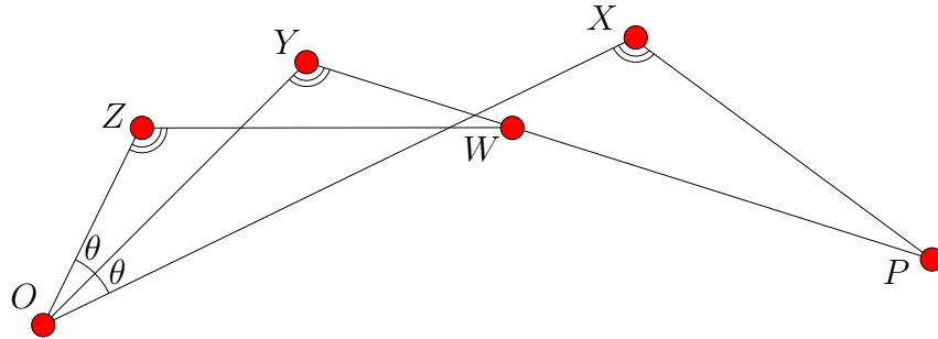
Figure 3-4: Kempe's reversor.
