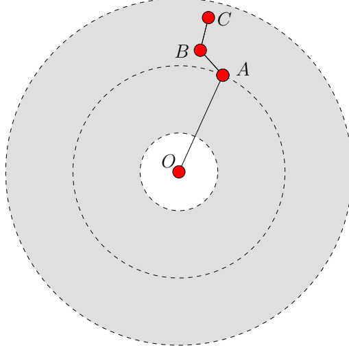
Figure 2-1: A linkage that does not rigidly construct its trace.
