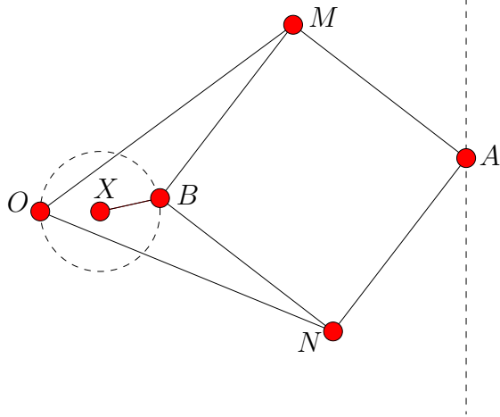
(a) Original Peaucellier inversor.
