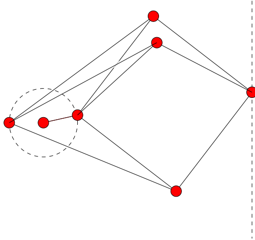
Figure 6-1: A 3-dimensional Peaucellier linkage.
