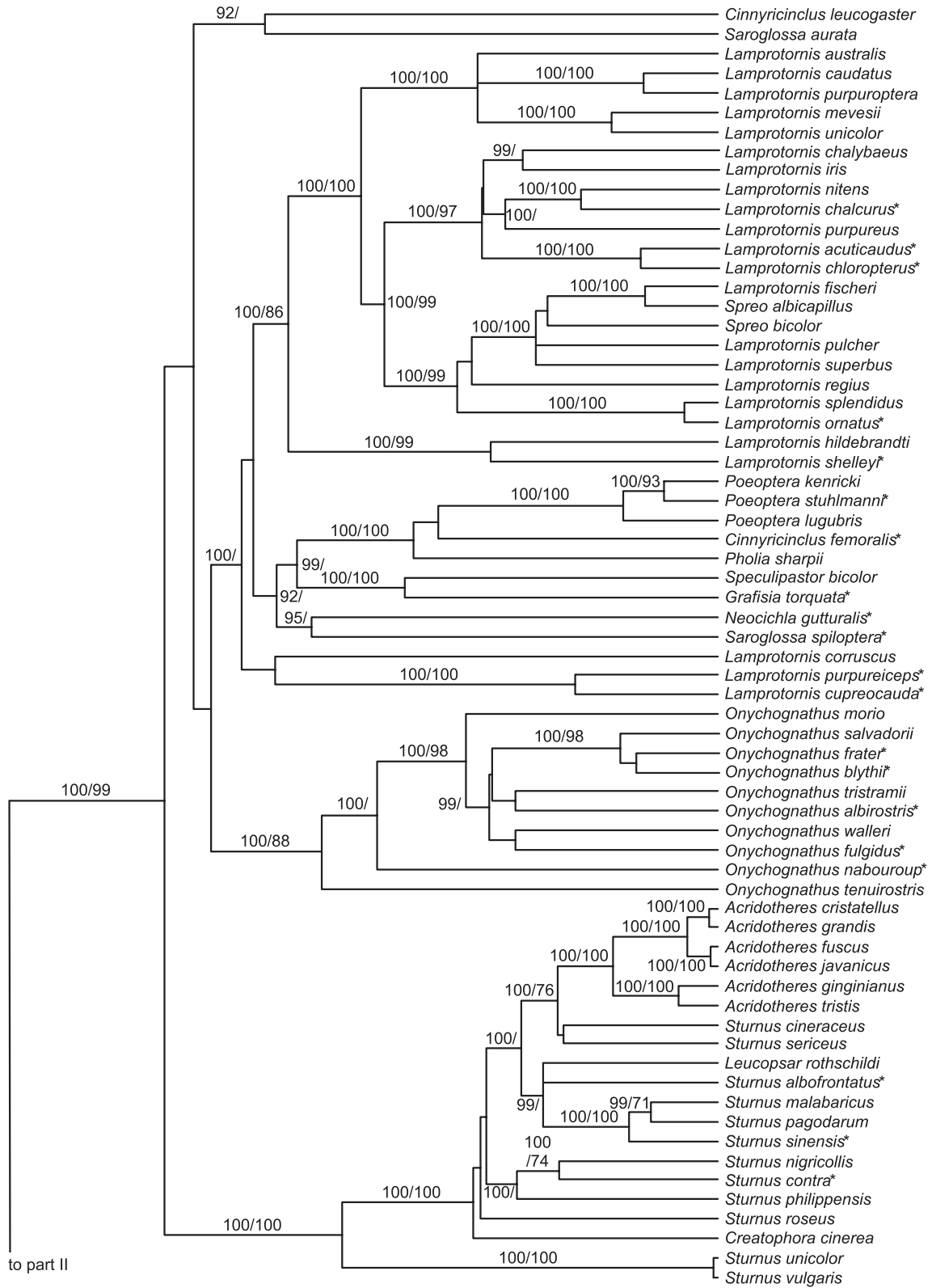
Fig. 2. Ultrametric Bayesian likelihood phylogeny for the Sturnidae and Mimidae based on mitochondrial protein-coding sequences (4116 nucleotides for most taxa; only 1041 bp NDII gene for taxa indicated with asterisks). Numbers above or adjacent to nodes indicate posterior probability values \geq 90 followed by maximum parsimony bootstrap scores \geq 70 ; missing values indicate scores below these thresholds. Owing to the dataset heterogeneity, branch lengths were calculated based on the NDII sequence region only. Tree was rooted to outgroups Bombycilla , Myadestes , and Catharus (not shown).
