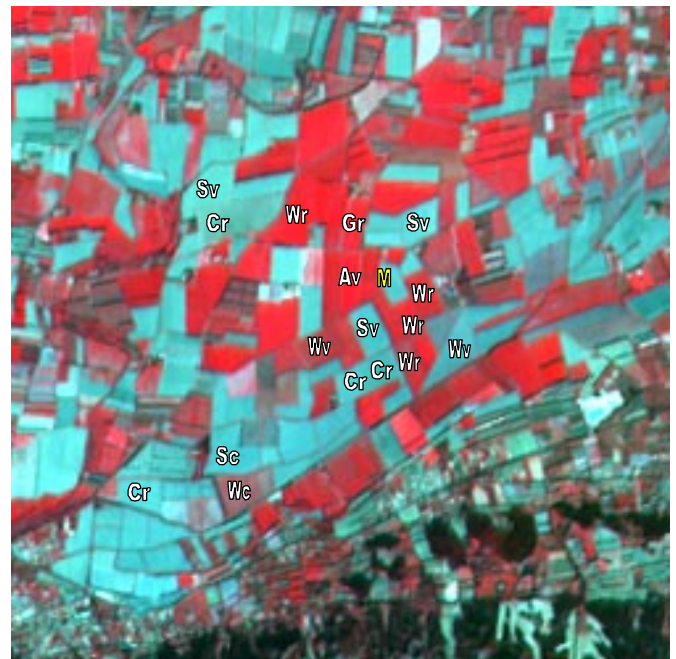
Figure 1: 5 km x 5 km SPOT-XS image acquired on March 25, 1997 over the Alpilles-ReSeDA site, along with ground-truth fields; M: meteorological site; W: wheat; S: sunflower; A: alfalfa; C: corn; G: grass; c: calibration fields; v: validation fields; r: remote sensing fields.
