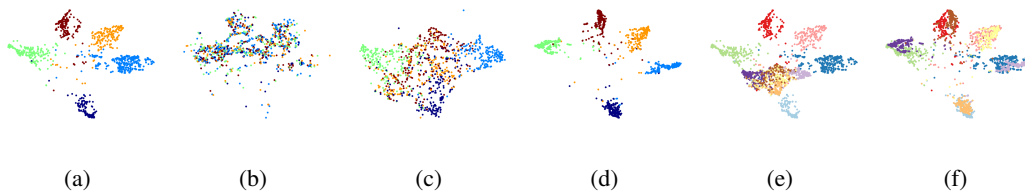
Figure 4: The t-SNE [68, 67] visualization of different feature embeddings. (a) Source domain embedding. (b) Target domain embedding using encoder trained with source domain domain. (c) Target domain embedding using encoder fine-tuned with target domain data. (d) Target domain embedding using encoder trained with our method. (e) An overlap of a and c. (f) An overlap of a and d. (best viewed in color and with zoom)
