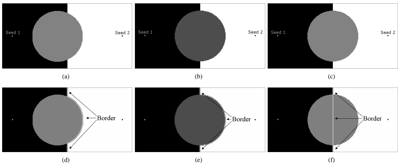
Fig. 7. This figure shows how ambiguous, unseeded regions are assigned to neighboring regions. (a,d) If the ambiguous region shares more surface area with one region, it is assigned to that region. (b,e) If the ambiguous region is closer in intensity to a neighboring region, it is assigned to that region. (c,f) If the ambiguous region is precisely centered between two regions with respect to both surface area and intensity, that region is divided in half. If more ambiguous regions are present (in a piecewise constant image), the ambiguous region will have the average probability of its neighbors, weighted by shared surface area and intensity difference.
