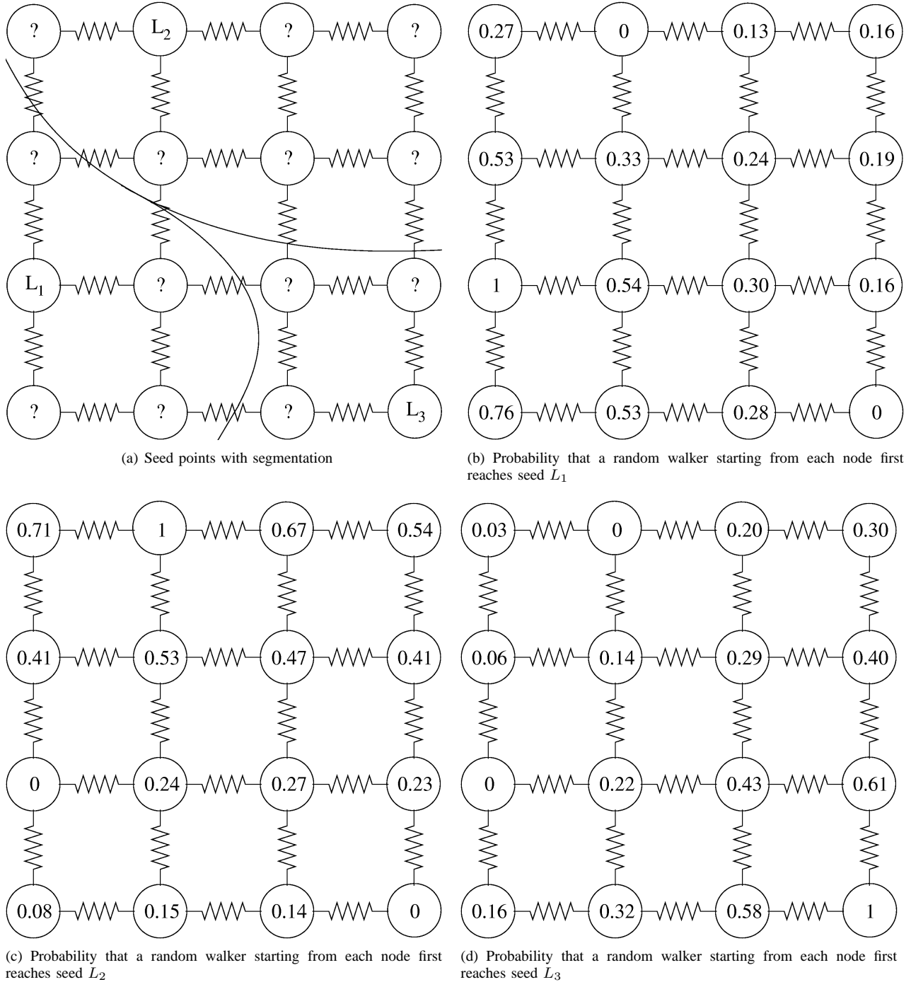
Fig. 1. Illustration of the approach to segmentation. With three seed points representing three different labels (denoted L_1, L_2, L_3 ), alternately fix the potential of each label to unity (i.e., with a voltage source tied to ground) and set to zero (i.e., ground) the remaining nodes. The electric potentials calculated represent the probability that a random walker starting at each node first reaches the seed point currently set to unity. Figure 1(a) shows the initial seed points and the segmentation resulting from assigning each node the label that corresponds to its greatest probability. For illustration, all the weights (resistors) were set to unity. In the case of an image, these resistors would be a function of the intensity gradient. The reader can verify that the probabilities at each node sum to unity (up to rounding).
