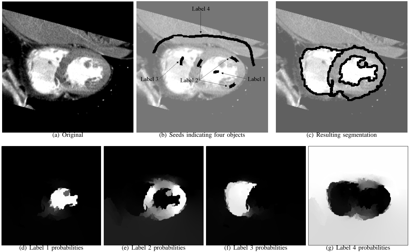
Fig. 2. Overview of segmentation computation. a) Original image to be segmented. b) User-placed seeds indicating a desired segmentation into four objects. d-g) Probabilities (potentials) obtained by solving (10) for each label. c) Segmentation obtained by assigning each pixel to the label for which a random walker is most likely to reach first. Each system required less than three seconds to solve using MATLAB.
