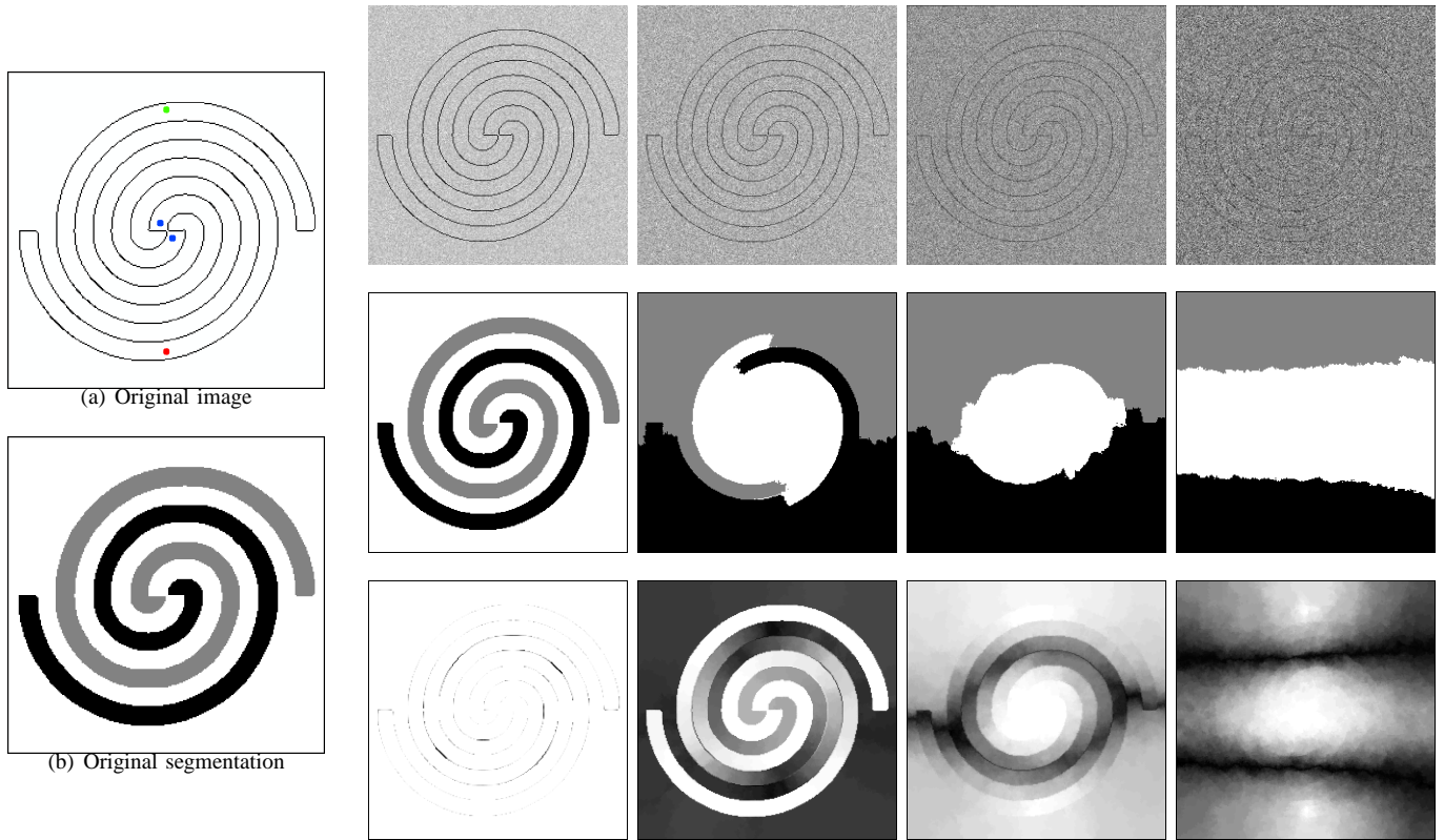
Fig. 6. This figure shows the characteristic response of the algorithm to noise. (a) An image consisting of two nested spirals was seeded with one seed in each spiral and two background seeds in the center (outside the spirals). (b) The initial (correct) segmentation. Increasing amounts of additive noise were then introduced into the image and the response of the algorithm was tracked. For each noise level, one hundred experiments were run in which the corrupted image was generated and the results were recorded. Top: A representative corrupted image, Middle: The “average” segmentation obtained from application of the algorithm, Bottom: The segmentation variability. An “average” segmentation was calculated by assigning the pixel to the label for which it was most often assigned over the one hundred trials. Segmentation variability of a pixel was measured by calculating the percentage of the trials for which the pixel was assigned the label from the “average” segmentation, with high percentage mapped to high intensity (white) and low percentage mapped to low intensity (black).
