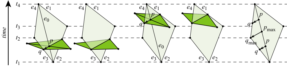
Fig. 9. An edge collapse in the triangle mesh M(t) (green) is equivalent to joining two faces of the hypermesh (light green).
