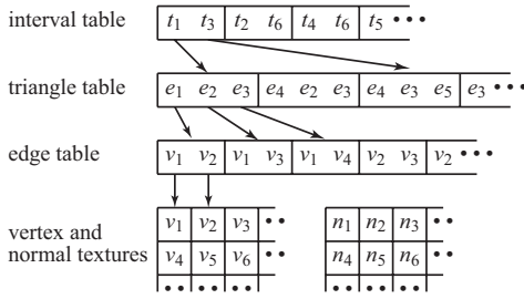
Fig. 8. Data structures used for GPU rendering.
