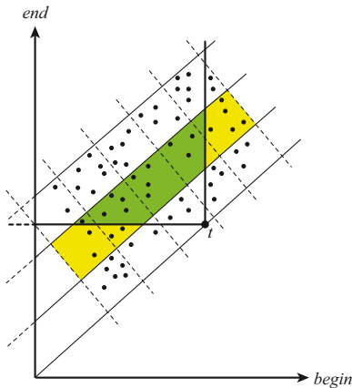
Fig. 10. Span space for the lifespans of the dynamic triangles: Each point represents an interval with the abscissa and ordinate referring to the start and end time. The three diagonal bands contain intervals with approximately the same length, with the short-living intervals close to the diagonal. The intervals in the second band that intersect with the current time t are shown in green.
