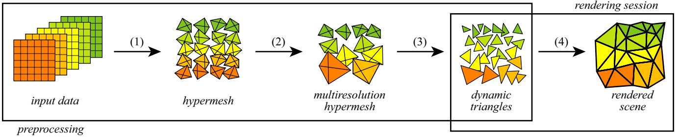
Fig. 2. Overview of the proposed framework. The preprocessing phase converts the input data into hypermeshes (1), builds a multiresolution model by utilizing quadric-error simplification (2), and converts the hypermesh into a set of dynamic triangles (3). This data structure is optimized for interactive rendering of the scene using the GPU (4).
