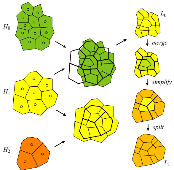
Fig. 6. Hierarchy of the V -partition (left) and the three steps of the coarsening algorithm (right).
