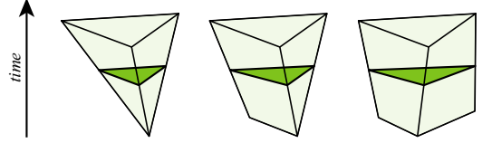
Fig. 11. Joining faces of the hypermesh as in Figure 9 generates non-tetrahedral elements.
