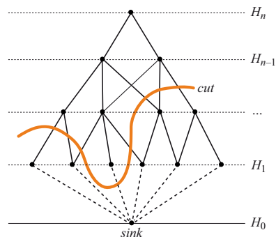
Fig. 7. A cut in the DAG.
