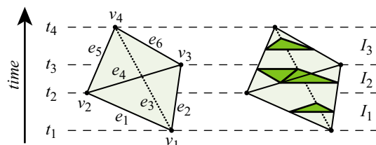
Fig. 4. Notation for a tetrahedron (left) and possible cases that occur when it is intersected with a plane (right).
