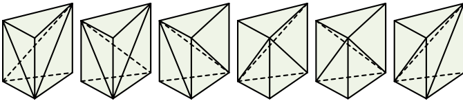
Fig. 5. Six different ways to split a prism into tetrahedra.
