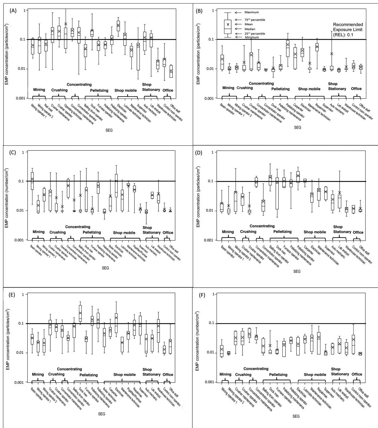
Fig. 1. Box plot of total EMP for each SEG in mines A–F (the horizontal line indicates the NIOSH REL for EMP = 0.1 particles cm -3 ).
