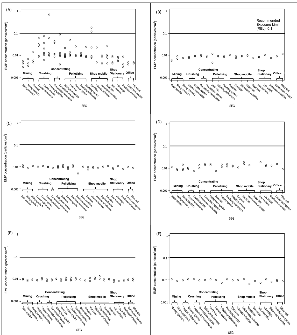
Fig. 2. Scatter plot of amphibole EMP for each SEG in mines A–F (the horizontal line indicates the NIOSH REL for EMP = 0.1 particles cm -3 ).
