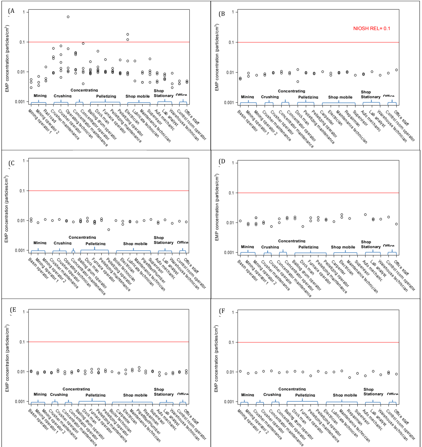
Figure 2. Scatter plot of amphibole EMP concentrations for each SEG in mines A-F (the horizontal line indicates the NIOSH REL for EMP = 0.1 particles/cm 3 )
