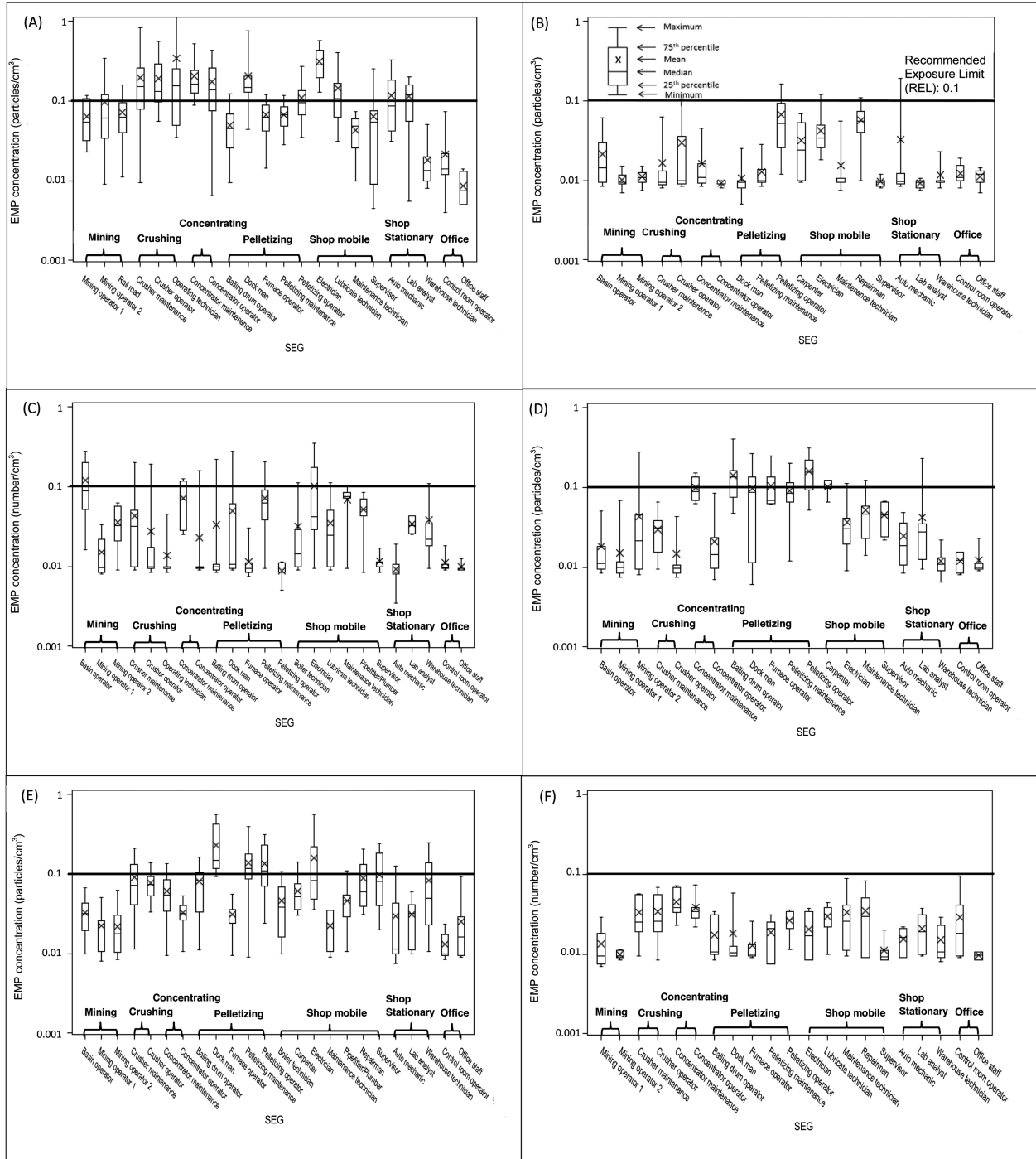
Figure 1. Box plot of total EMP for each SEG in mines A-F (the horizontal line indicates the NIOSH REL for EMP = 0.1 particles cm -3 ) 1 .
