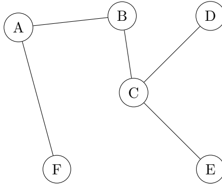
Figure 5.15: A free tree.
