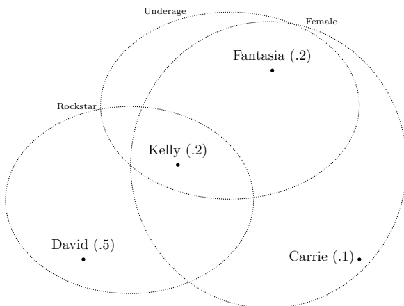
Figure 4.1: Various events, and their overlap.
