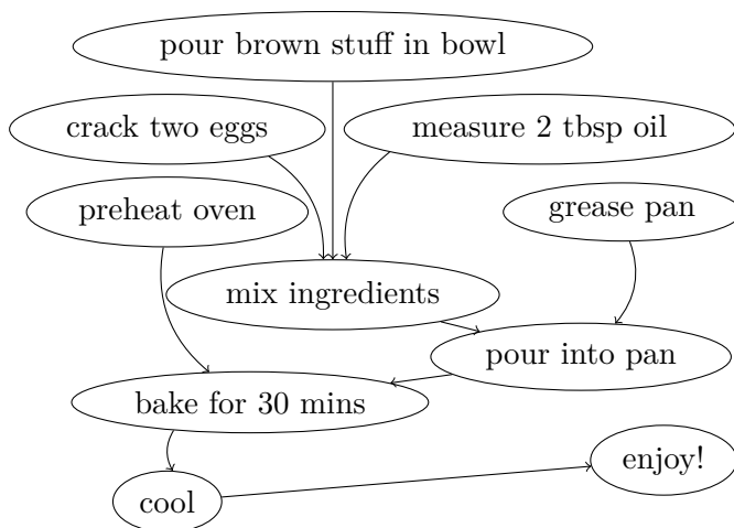
Figure 5.4: A DAG.
