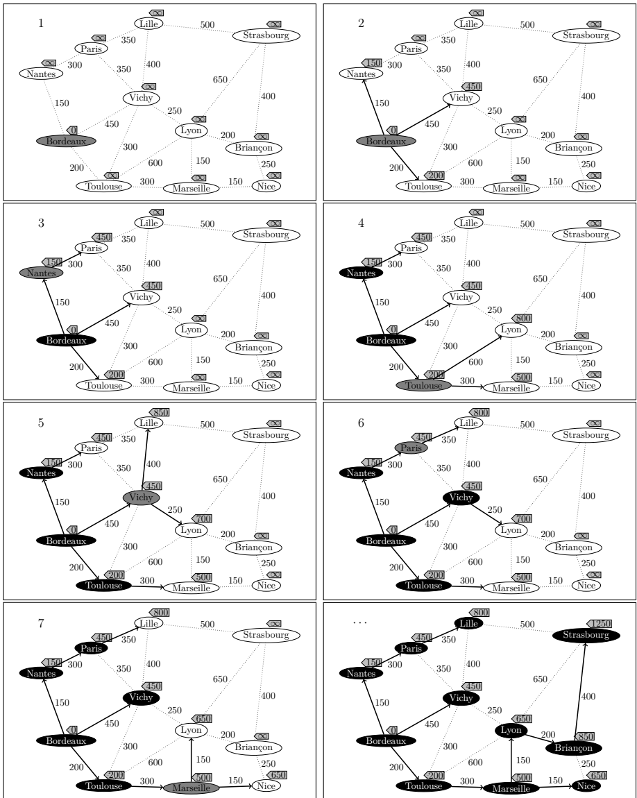
Figure 5.13: The stages of Dijkstra’s shortest-path algorithm. The “current node” is shown in grey, with visited nodes (whose best paths and shortest distances have been unalterably determined) in black. The sign next to each node shows the tentative shortest distance to that node from Bordeaux.
