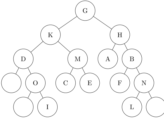
Figure 5.21: A full binary tree.
