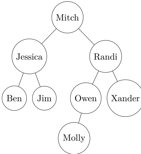
Figure 5.24: A binary search tree.
