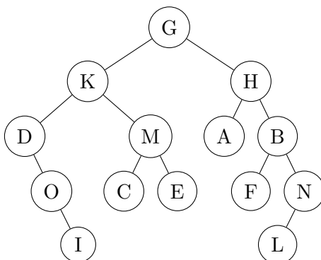
Figure 5.17: A binary tree.
