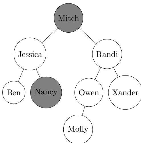
Figure 5.25: NOT a binary search tree, though it looks like one at first glance. (Notice Nancy and Mitch)
