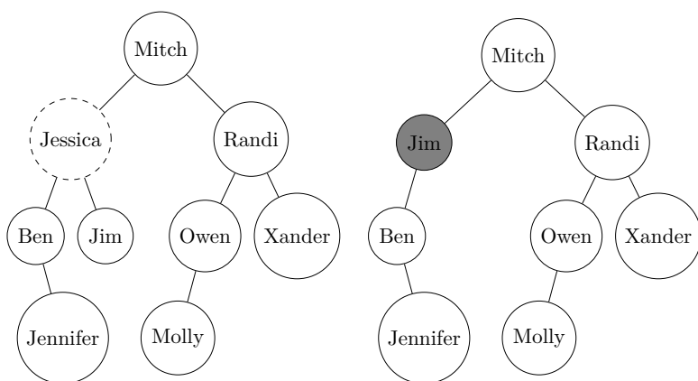
Figure 5.28: The BST after removing Jessica correctly.
