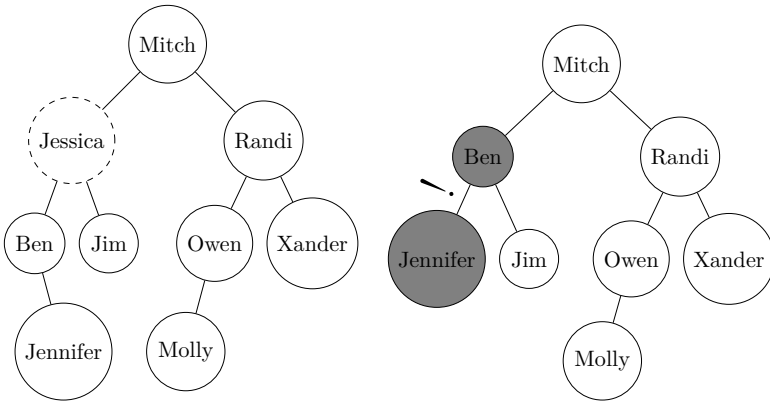
Figure 5.27: A wrong (non)-BST after removing Jessica incorrectly.
