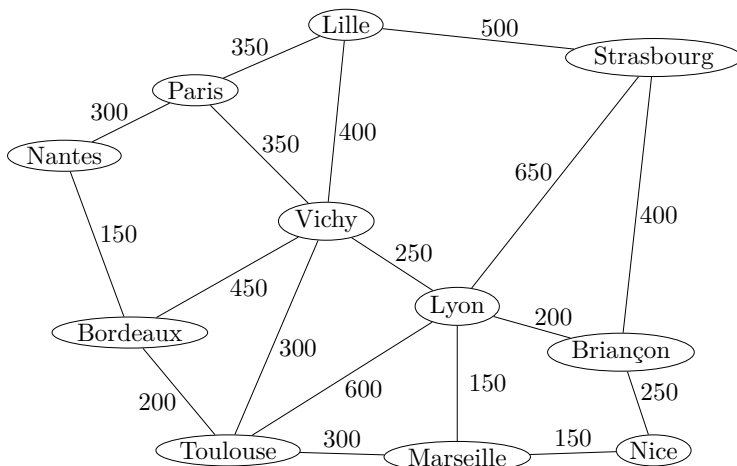
Figure 5.12: A weighted graph, through which we desire to find the shortest path from Bordeaux to Strasbourg.
