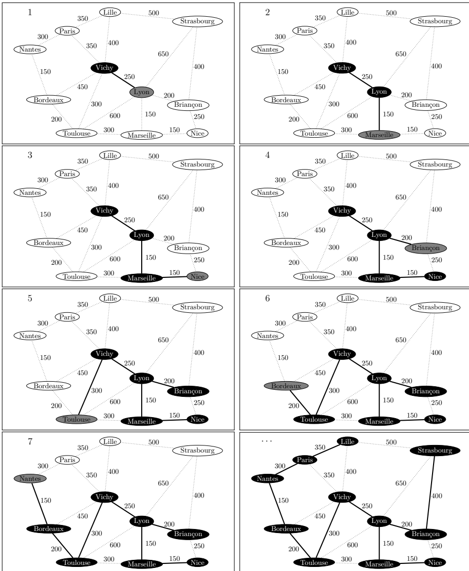
Figure 5.14: The stages of Prim's minimal connecting edge set algorithm. Heavy lines indicate edges that have been (irrevocably) added to the set.
