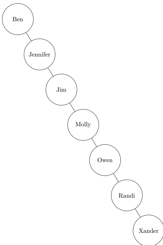
Figure 5.30: An incredibly bad, but still technically legit, BST.
