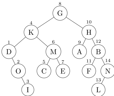
Figure 5.20: The order of node visitation in in-order traversal.
