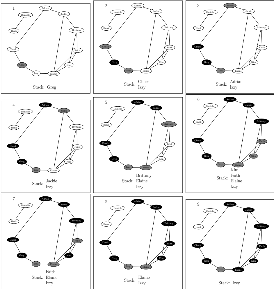
Figure 5.11: The stages of depth-first traversal. Marked nodes are grey, and visited nodes are black. The order of visitation is: G, C, A, J, B, K, F, E, I.
