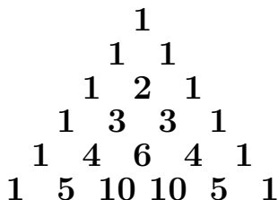
Figure 6.1: The first six rows of Pascal’s triangle.
