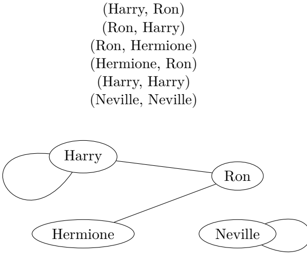
Figure 5.7: A graph depicting a symmetric endorelation.
