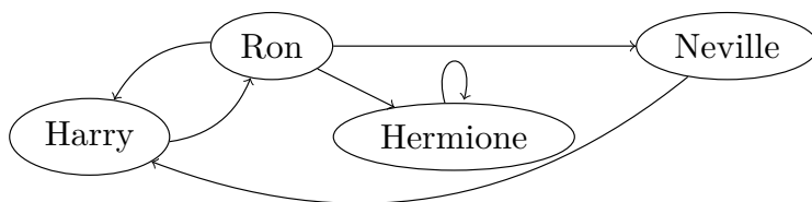
Figure 5.6: A graph depicting a endorelation.
