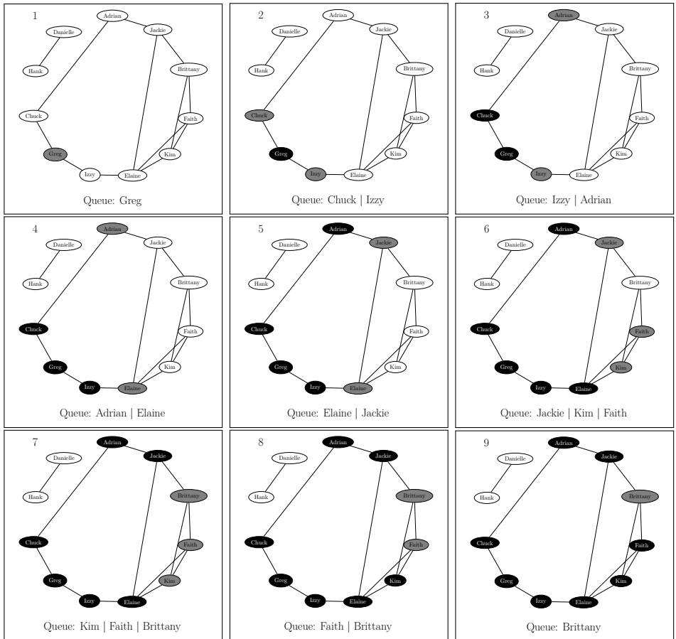
Figure 5.9: The stages of breadth-first traversal. Marked nodes are grey, and visited nodes are black. The order of visitation is: G, C, I, A, E, J, K, F, B.
