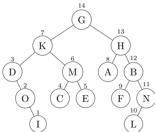
Figure 5.19: The order of node visitation in post-order traversal.
