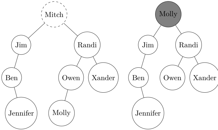
Figure 5.29: The BST after removing Mitch.
