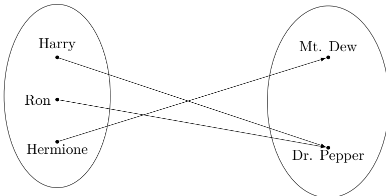
Figure 3.1: A function represented graphically.
