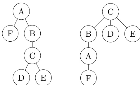
Figure 5.16: Two different rooted trees with the same vertices and edges.
