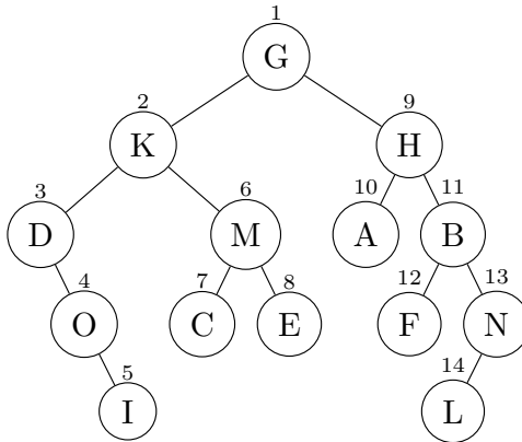
Figure 5.18: The order of node visitation in pre-order traversal.
