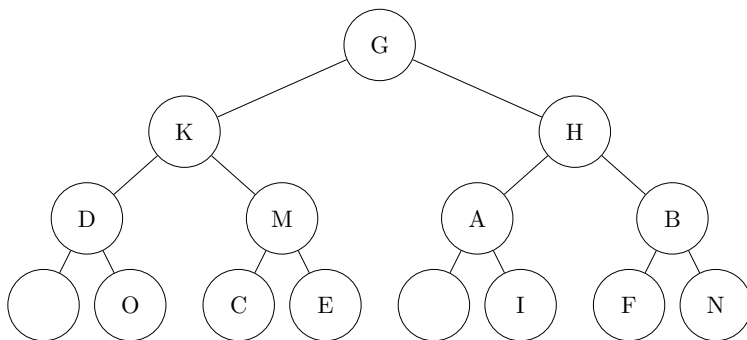
Figure 5.23: A “perfect” binary tree.
