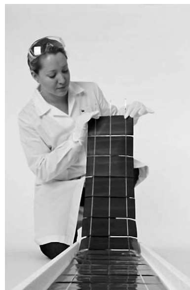
Figure 13. The new PowerFlex Solar Strings thin-film flexible photovoltaic material by Global Solar Energy Inc. (photo courtesy of Global Solar Energy Inc.).
