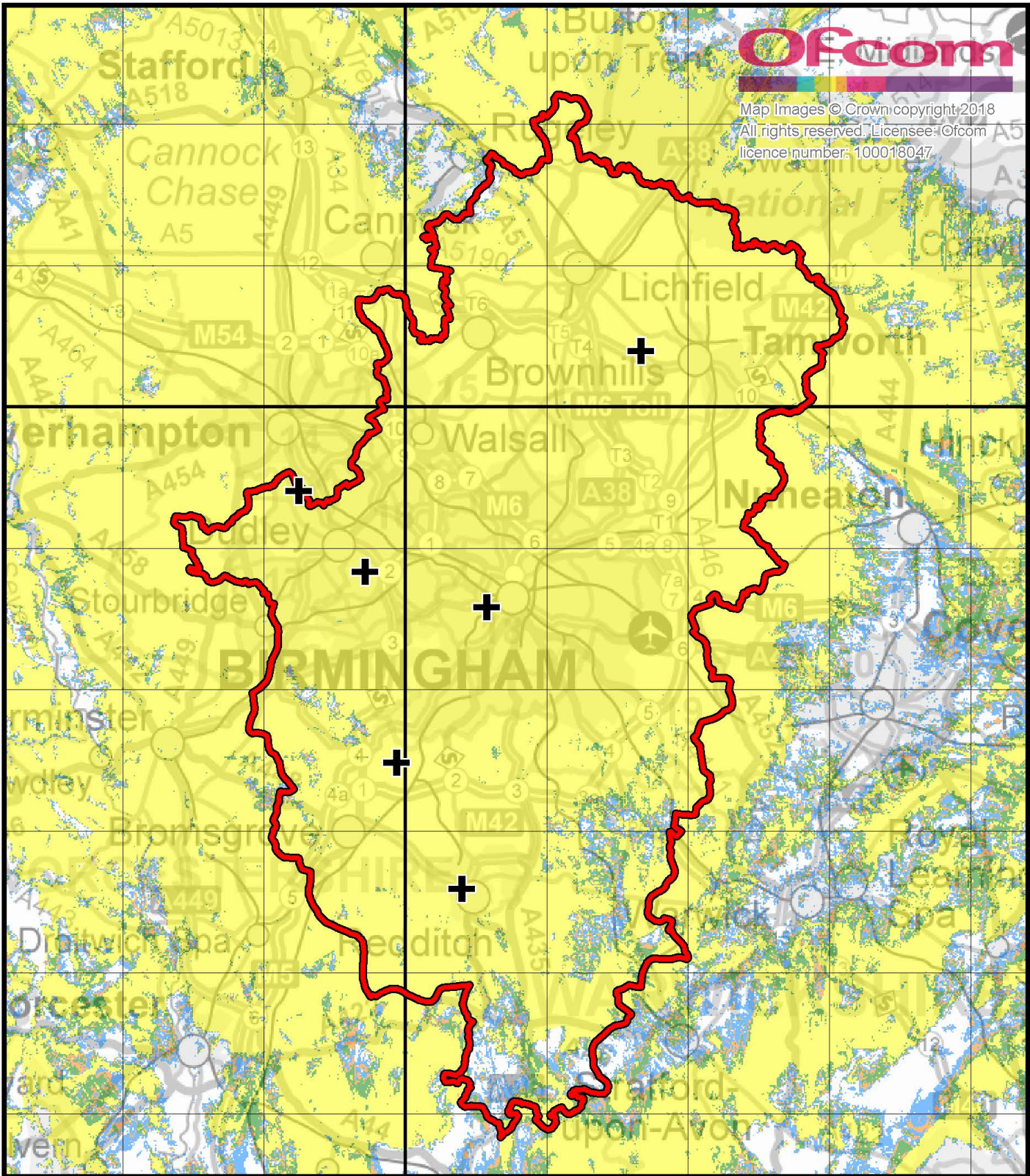
Birmingham local DAB multiplex service (CE Digital). Mobile coverage, normal propagation conditions. July 2018.
