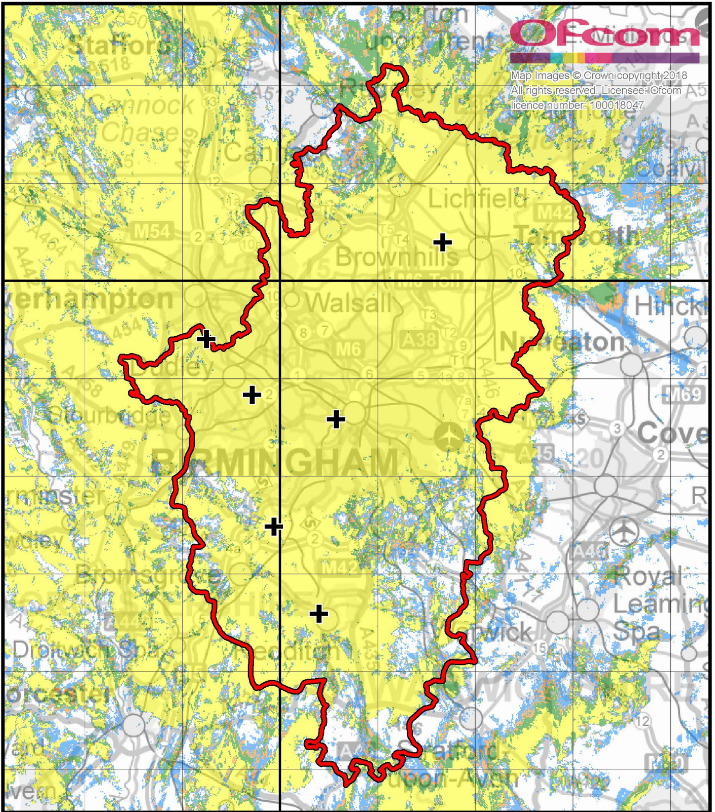
Birmingham local DAB multiplex service (CE Digital). Mobile coverage, enhanced propagation conditions. July 2018.
