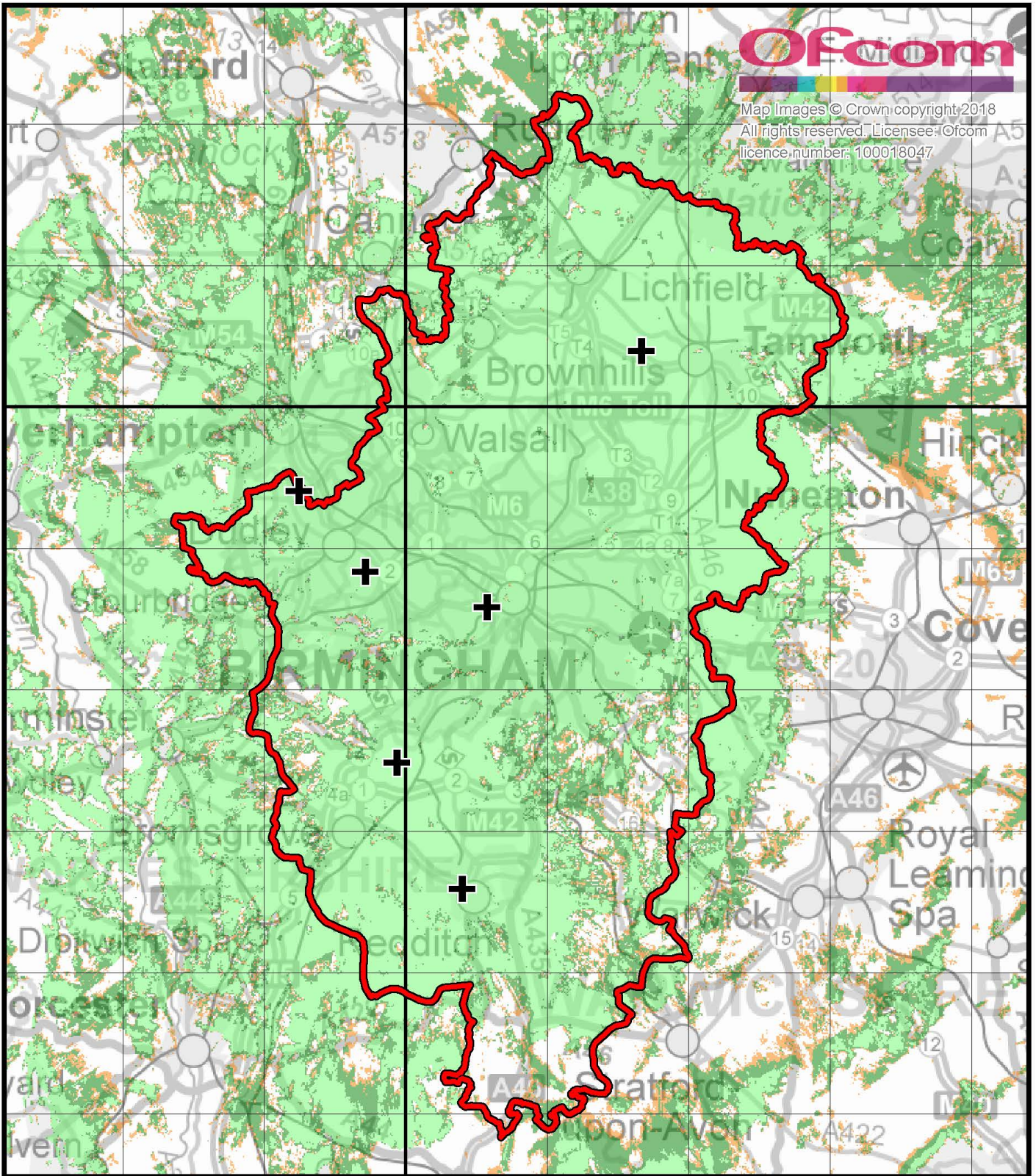
Birmingham local DAB multiplex service (CE Digital). Indoor coverage, normal propagation conditions. July 2018.
