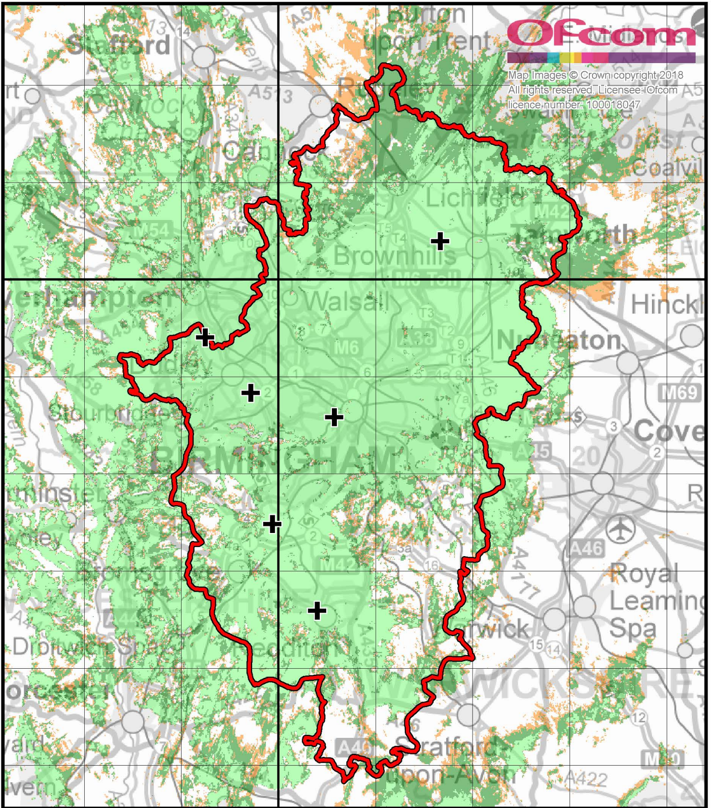
Birmingham local DAB multiplex service (CE Digital). Indoor coverage, enhanced propagation conditions. July 2018.
