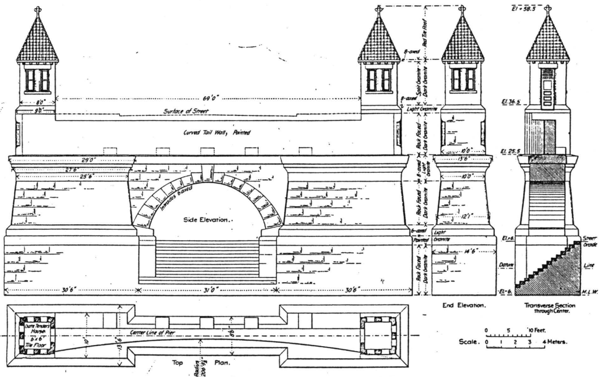
fig. E: 155th Street Viaduct (1921)
