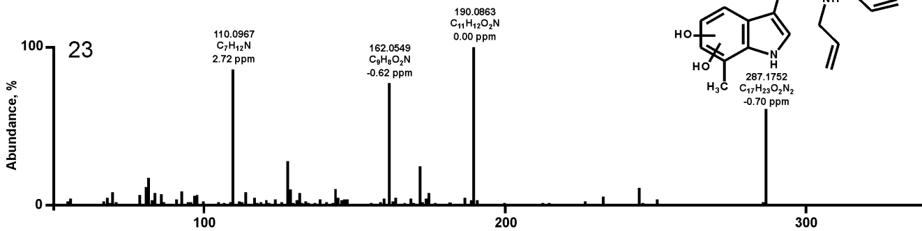
7-Me-DALT-M (di-HO-aryl-); RT 3.7
