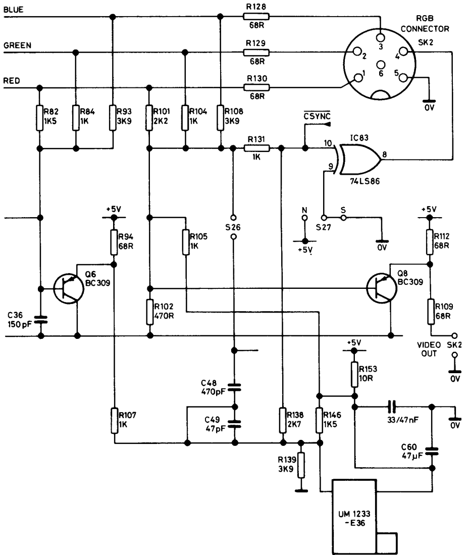
Video outputs
