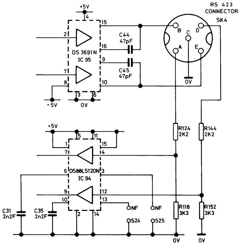
RS423 interface
