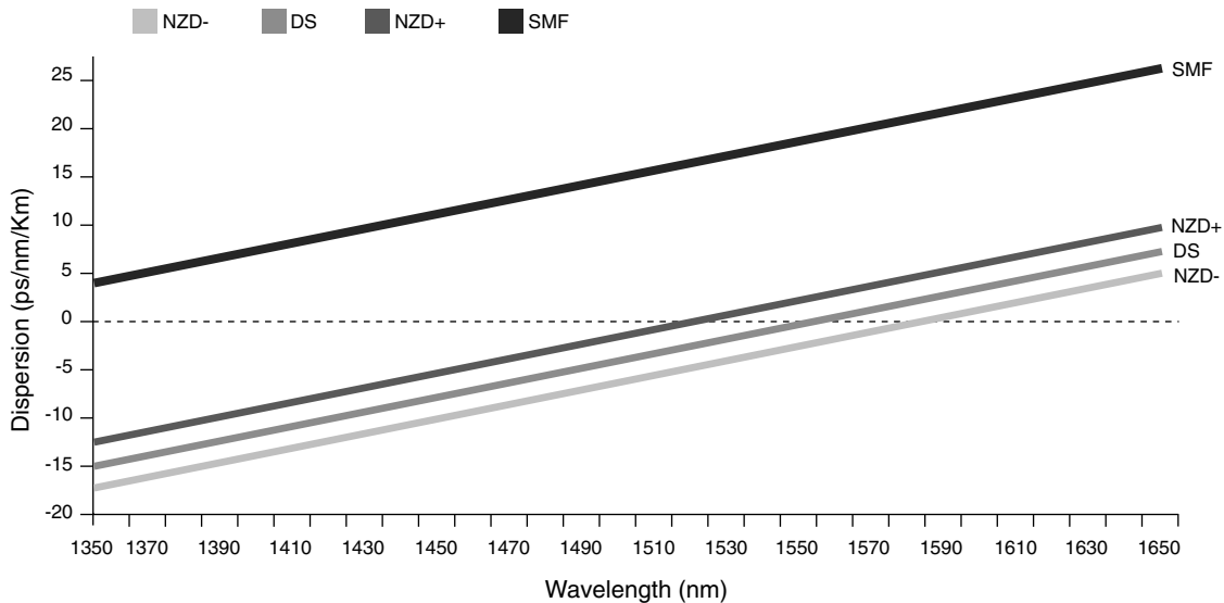
Figure 3-14 Fiber Dispersion Slopes
