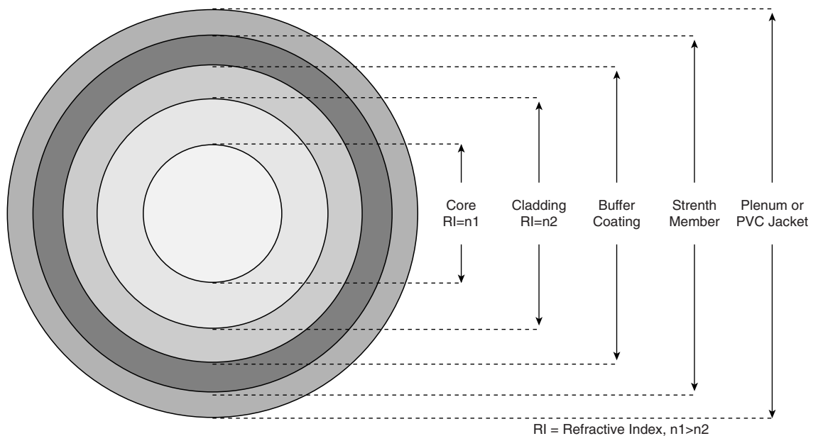
Figure 3-1 Cross Section of a Fiber-Optic Cable
