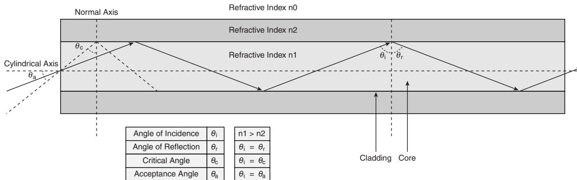
Figure 3-2 Total Internal Reflection
