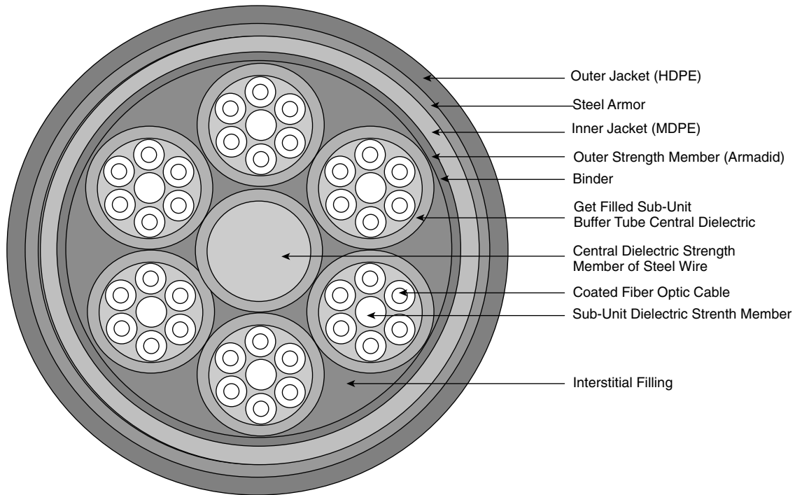
Figure 3-7 Cross Section of an Armored Outside-Plant Cable
