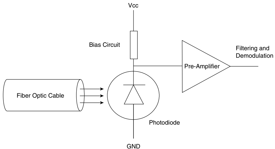
Figure 3-19 Schematic of an Optical Receiver
