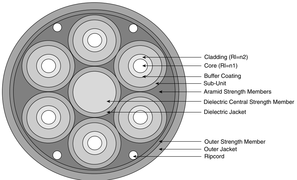
Figure 3-6 Cross Section of Inside-Plant Cables
