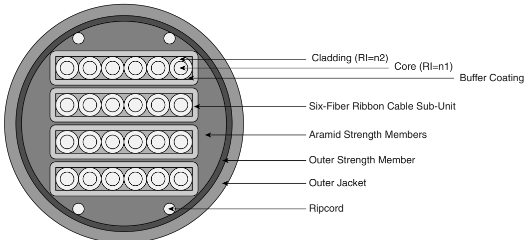
Figure 3-5 Inside Plant Ribbon-Cable System
