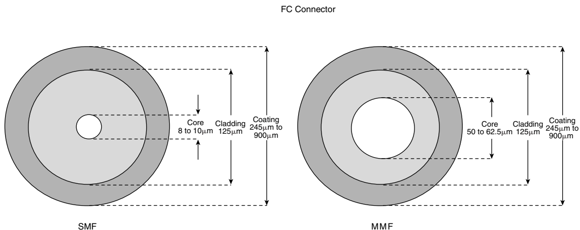
Figure 3-4 Optical-Cable Construction
