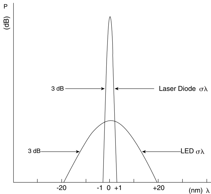
Figure 3-18 LED and LD Spectral Widths
