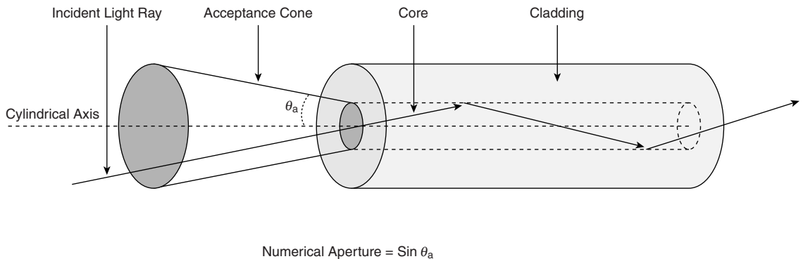
Figure 3-3 Acceptance Cone
