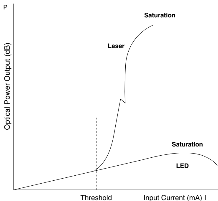
Figure 3-17 LED and LD P-I Characteristics
