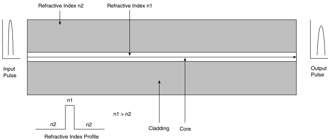
Figure 3-9 Single-Mode Step Index
