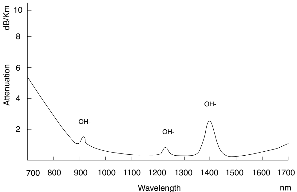
Figure 3-12 Attenuation Versus Wavelength
