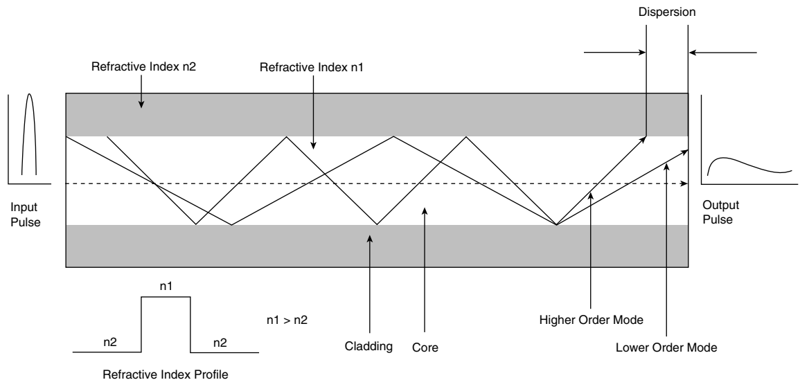
Figure 3-8 Multimode Step Index
