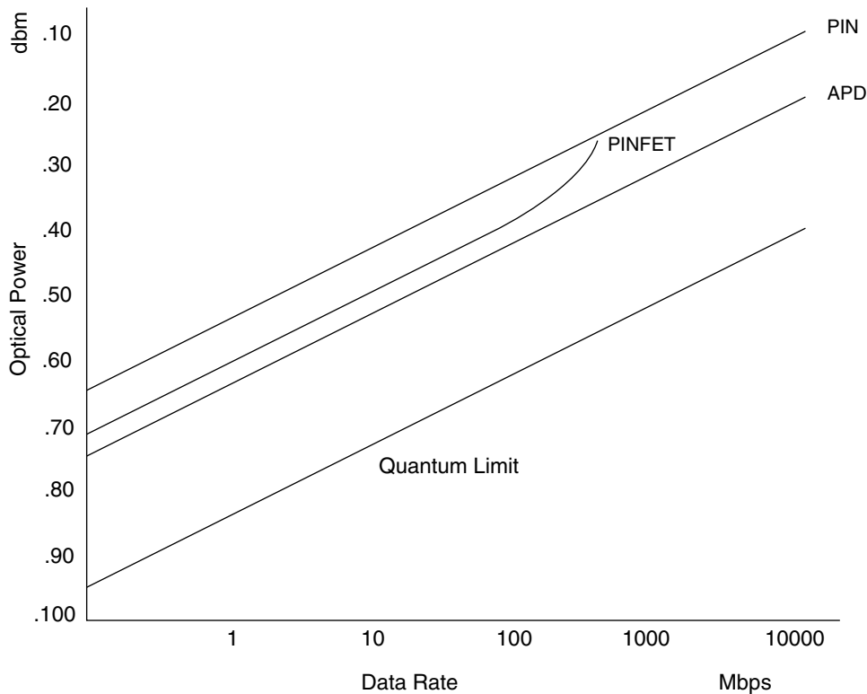
Figure 3-20 Receiver Sensitivity Curves
