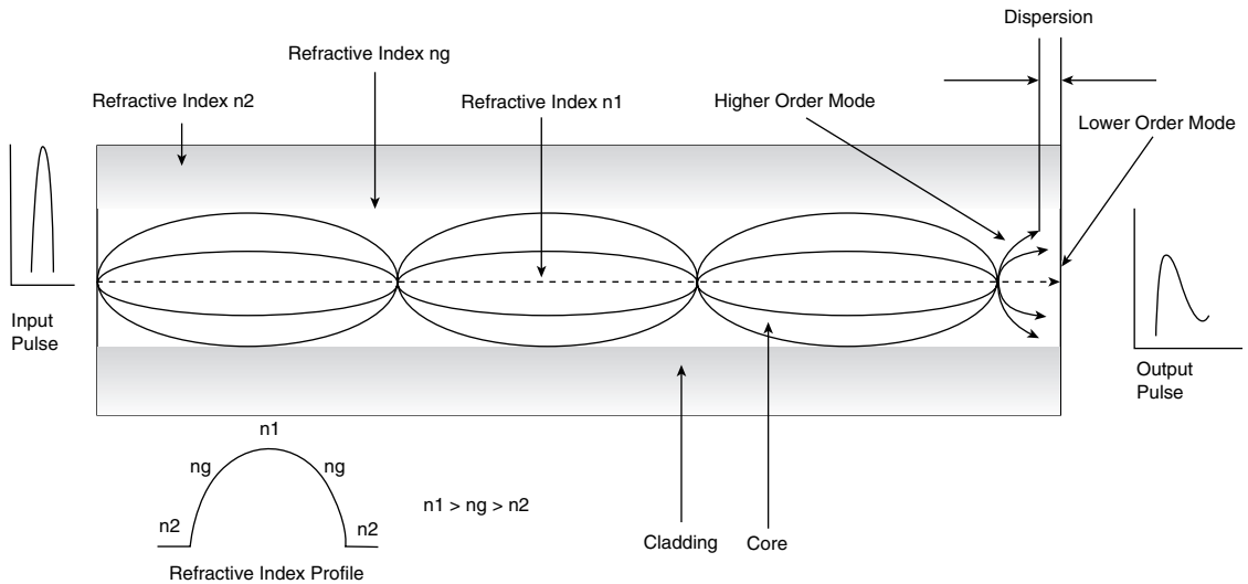
Figure 3-11 Multimode Graded Index
