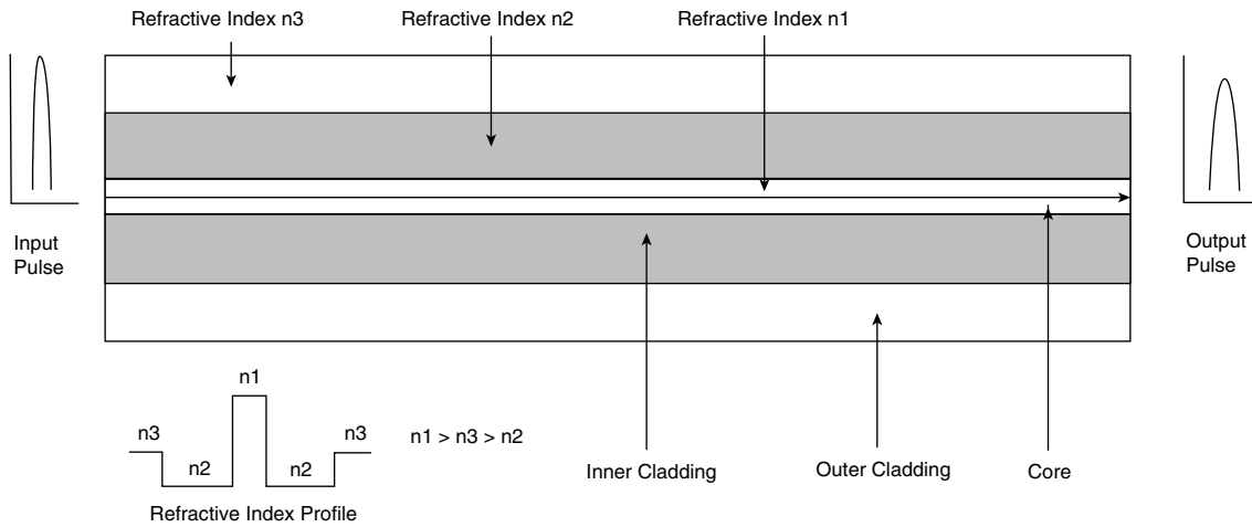
Figure 3-10 Single-Mode Dual-Step Index
