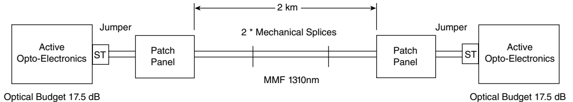
Figure 3-21 MMF Span Analysis
