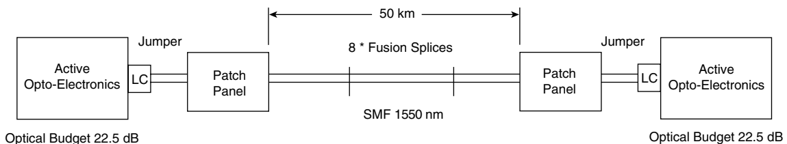
Figure 3-22 SMF Link-Budget Example
