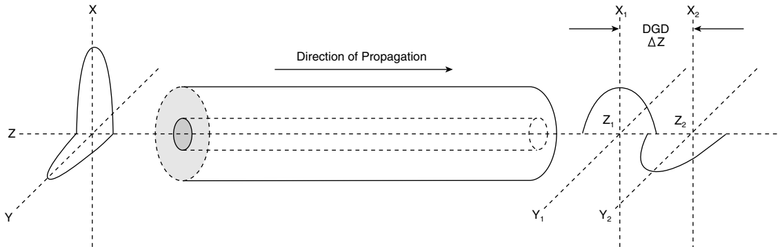
Figure 3-13 Polarization Mode Dispersion
