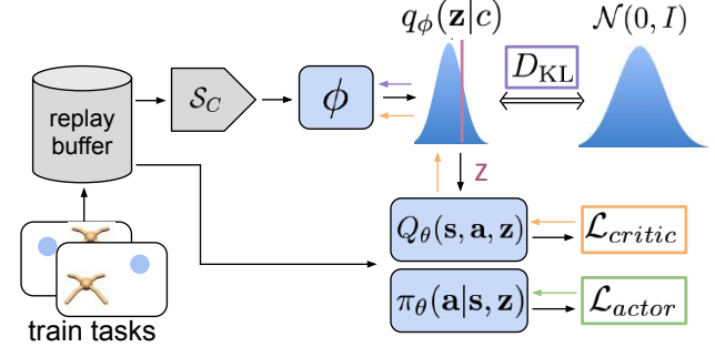
Figure 2. Meta-training procedure. The inference network q_\phi uses context data to infer the posterior over the latent context variable Z , which is passed as an input to the actor and critic. q_\phi is optimized with gradients from the critic as well as from an information bottleneck on Z . De-coupling the data sampling strategies for context ( S_C ) and actor-critic batches is important for off-policy learning, see ablation in Section 6.3.
