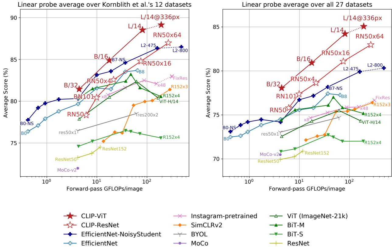
Figure 6. Linear probe performance of CLIP models in comparison with SOTA computer vision models, including EfficientNet (Tan & Le, 2019; Xie et al., 2020), MoCo (Chen et al., 2020b), Instagram-pretrained ResNeXt models (Mahajan et al., 2018; Touvron et al., 2019), BiT (Kolesnikov et al., 2019), ViT (Dosovitskiy et al., 2020), SimCLRv2 (Chen et al., 2020a), BYOL (Grill et al., 2020), and the original ResNet models (He et al., 2016b). (Left) Scores are averaged over 12 datasets studied by Kornblith et al. (2019). (Right) Scores are averaged over 27 datasets that contain a wider variety of distributions. Dotted lines indicate models fine-tuned or evaluated on images at a higher-resolution than pre-training. Please see supplementary material for individual model scores for each dataset.
